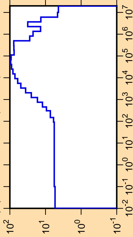
\Delta\mu/\mu vs. E for ^{189}\text{Pb}(\text{mt251})
