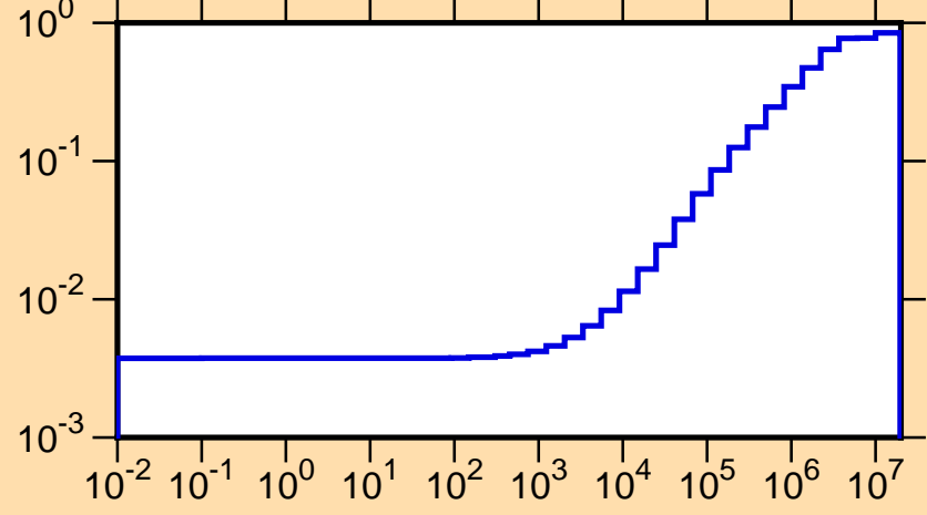
\mu vs. E for ^{189}\text{Pb}(\text{mt251})
