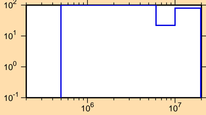
\Delta\sigma/\sigma vs. E for ^{189}\text{Pb}(n,n\text{cont.})
