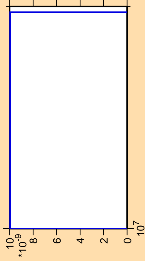
\Delta\sigma/\sigma vs. E for ^{189}\text{Pb} (mt 11)
