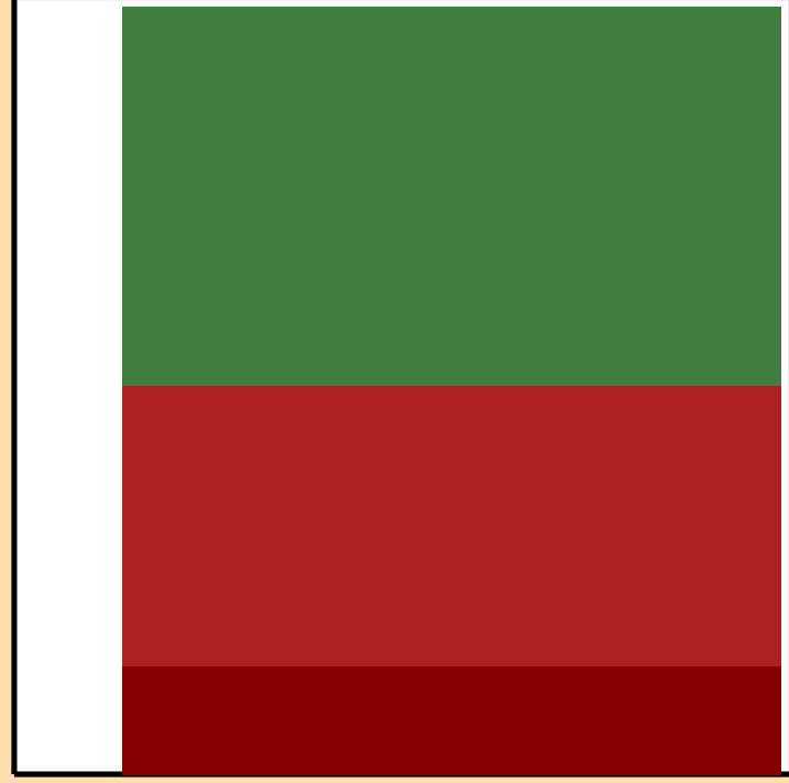
\Delta\sigma/\sigma vs. E for ^{189}\text{Pb}(n,2n)
