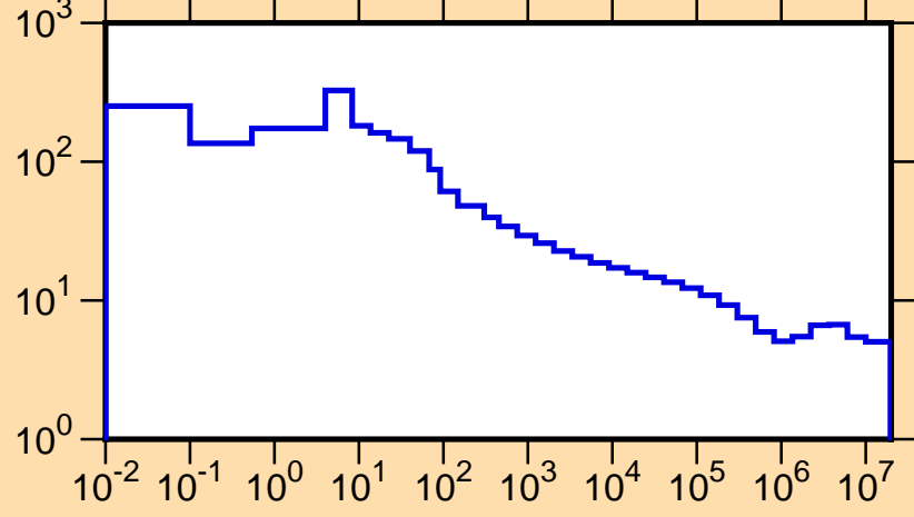
\sigma vs. E for ^{189}\text{Pb}(n,\text{tot.})
