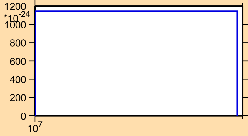
\sigma vs. E for ^{189}\text{Pb} (mt 11)
