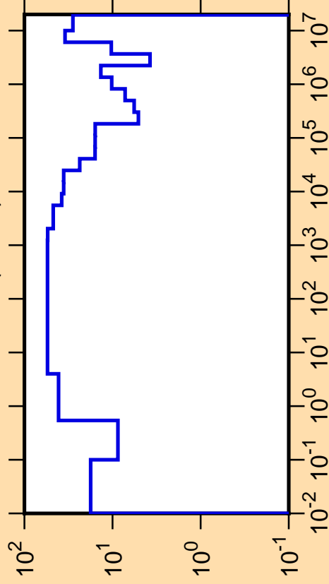
\Delta\sigma/\sigma vs. E for ^{189}\text{Pb}(n,\text{tot.})
