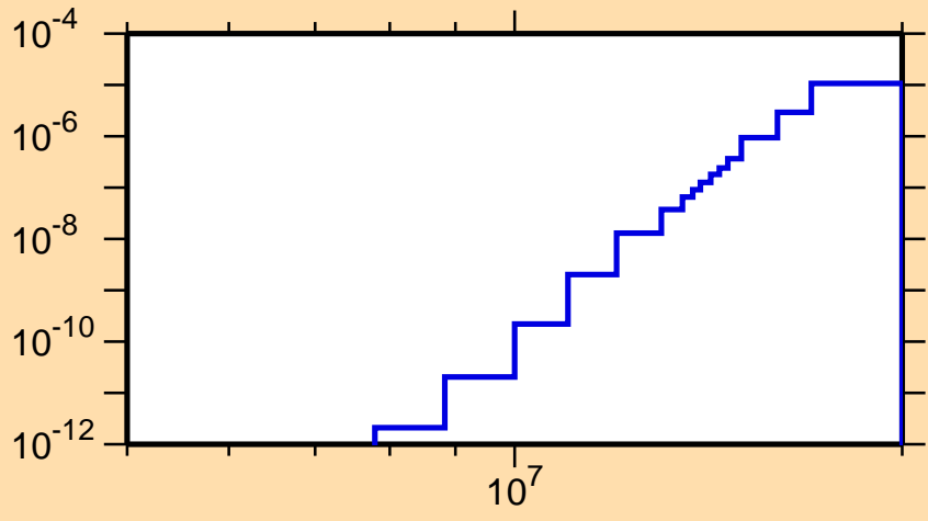
\sigma vs. E for ^{190}\text{Pb}(n,\text{He3})
