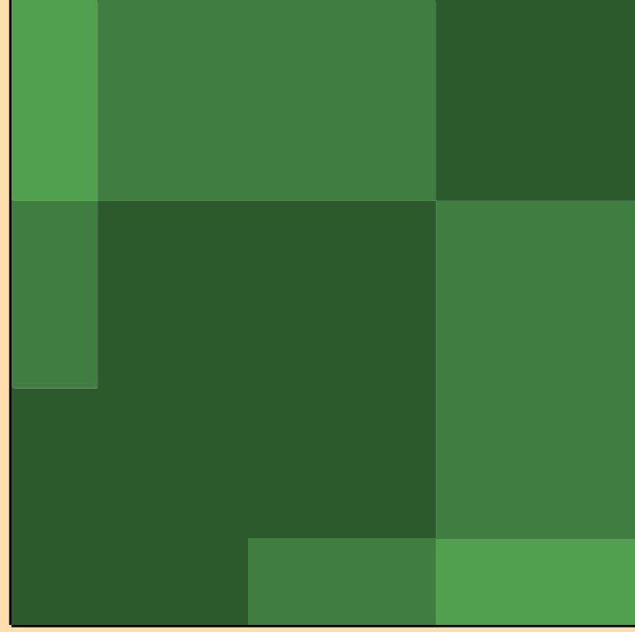
\sigma vs. E for ^{190}\text{Pb}(n,2n)
