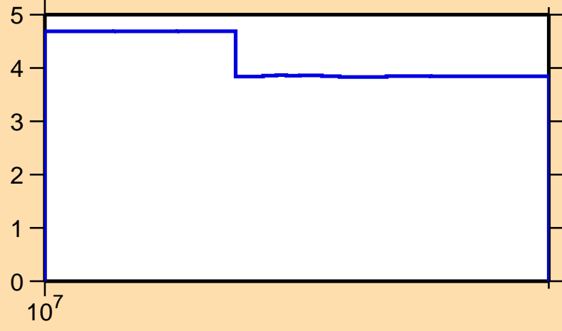
\Delta\sigma/\sigma vs. E for ^{190}\text{Pb}(n,\text{nonel.})
