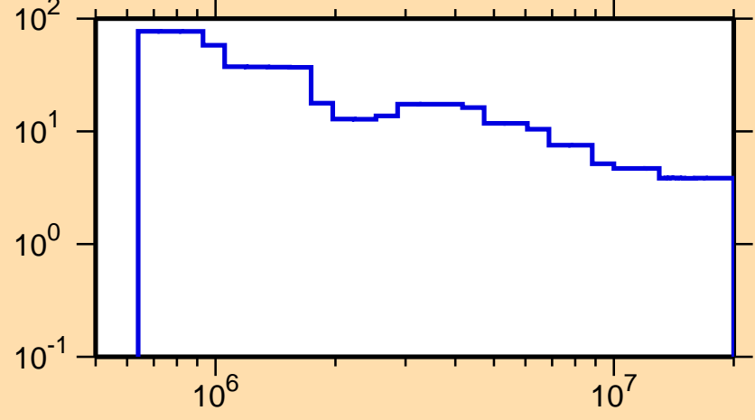
\Delta\sigma/\sigma vs. E for ^{190}\text{Pb}(n,\text{nonel.})
