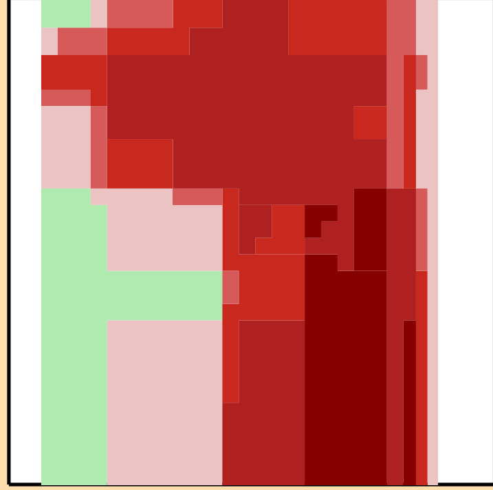
\Delta\sigma/\sigma vs. E for ^{190}\text{Pb}(n,n_1)
