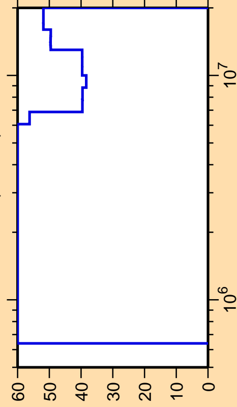
\Delta\sigma/\sigma vs. E for ^{190}\text{Pb}(n,\text{inel.})
