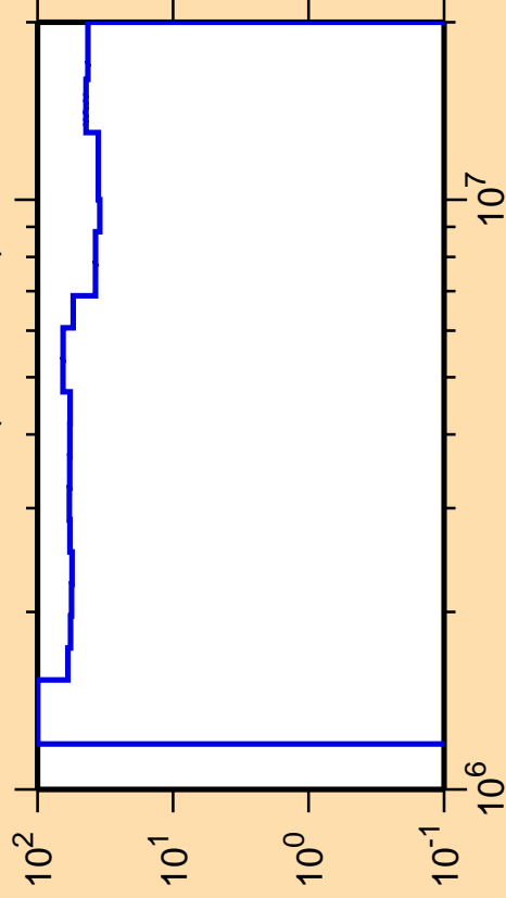
\Delta\sigma/\sigma vs. E for ^{190}\text{Pb}(n,n\text{cont.})
