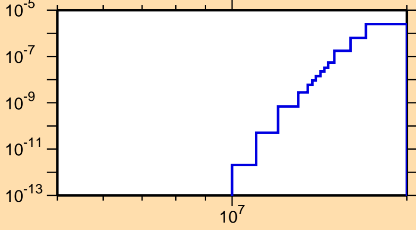
\sigma vs. E for ^{190}\text{Pb}(\text{mt } 45)
