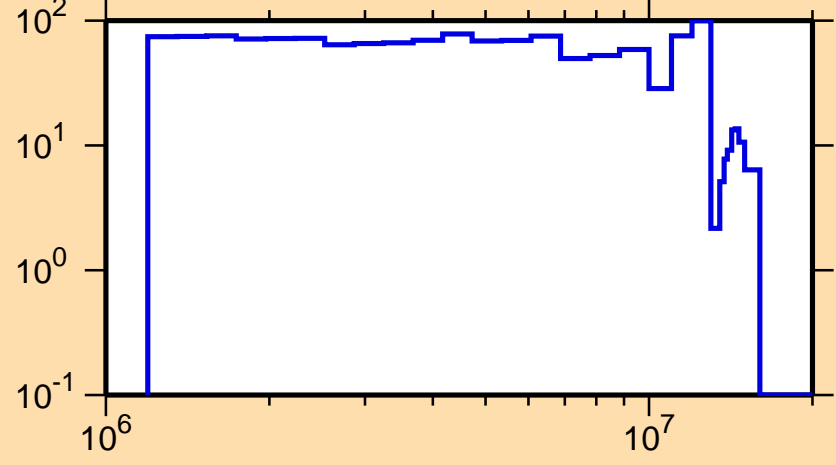
\Delta\sigma/\sigma vs. E for ^{190}\text{Pb}(n,n_1)
