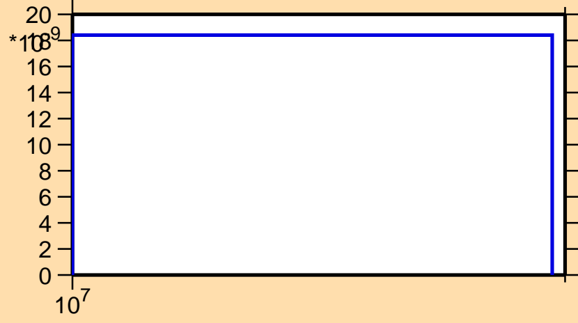
\sigma vs. E for ^{190}\text{Pb}(n,3n)
