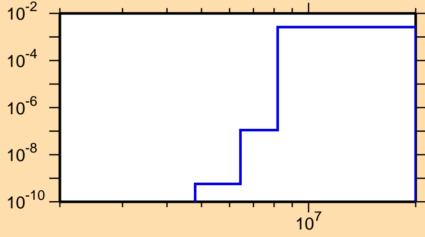
\sigma vs. E for ^{190}\text{Pb}(n,d)
