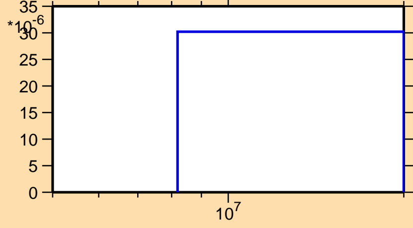
\sigma vs. E for ^{190}\text{Pb}(n,t)
