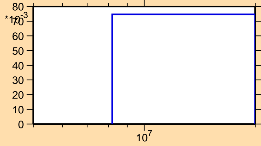
\sigma vs. E for ^{190}\text{Pb}(n,2n)
