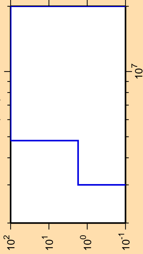
\Delta\sigma/\sigma vs. E for ^{190}\text{Pb}(n,d)
