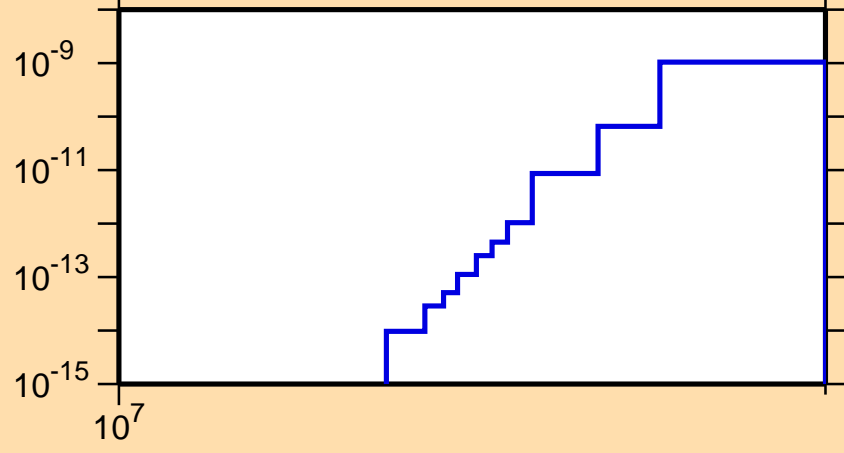
\sigma vs. E for ^{191}\text{Pb}(\text{mt } 34)
