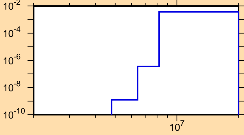
\sigma vs. E for ^{191}\text{Pb}(n,d)
