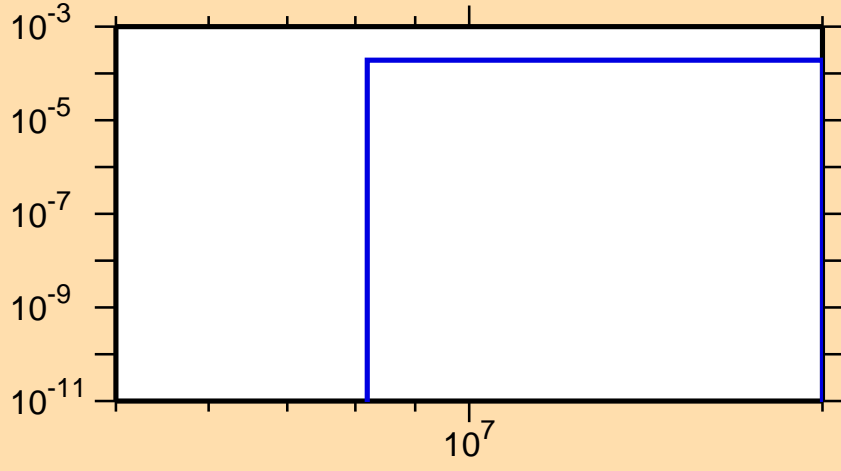
\sigma vs. E for ^{191}\text{Pb}(n,t)
