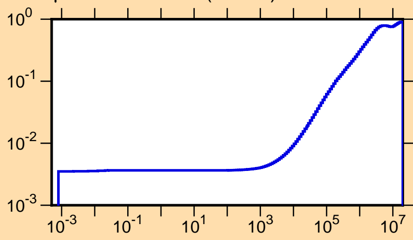
\mu vs. E for ^{192}\text{Pb}(\text{mt251})
