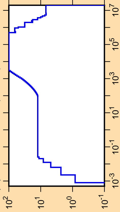
\Delta\mu/\mu vs. E for ^{192}\text{Pb}(\text{mt251})
