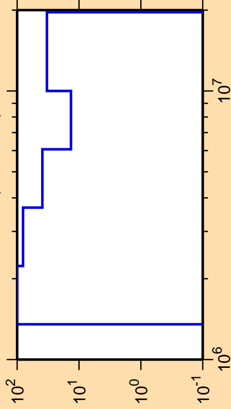
\Delta\sigma/\sigma vs. E for ^{192}\text{Pb}(n,n\text{cont.})
