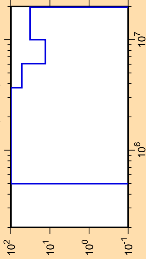
\Delta\sigma/\sigma vs. E for ^{192}\text{Pb}(n,\text{inel.})
