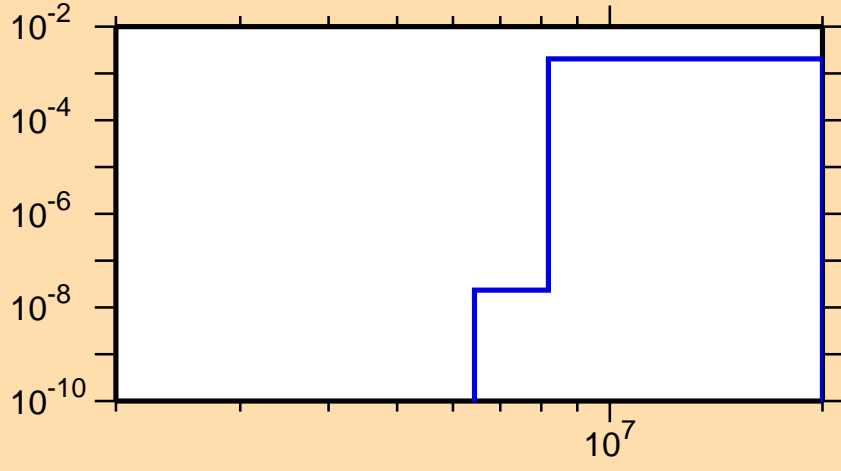
\sigma vs. E for ^{192}\text{Pb}(n,d)
