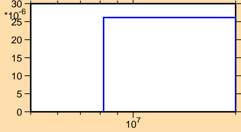
\sigma vs. E for ^{192}\text{Pb}(n,t)
