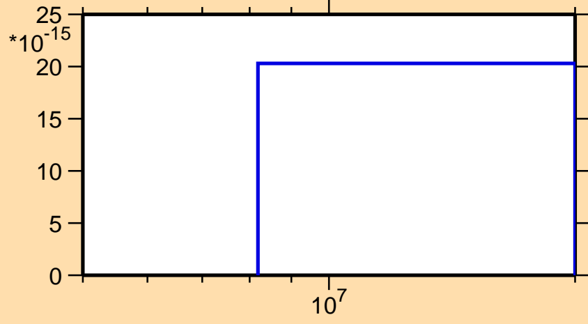
\sigma vs. E for ^{192}\text{Pb} (mt 34)
