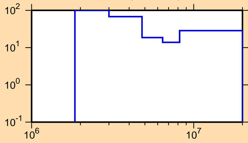
\Delta\sigma/\sigma vs. E for ^{192}\text{Pb}(n,ncont.)
