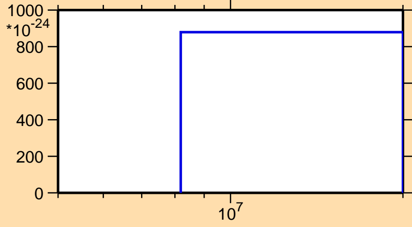
\sigma vs. E for ^{192}\text{Pb} (mt 11)
