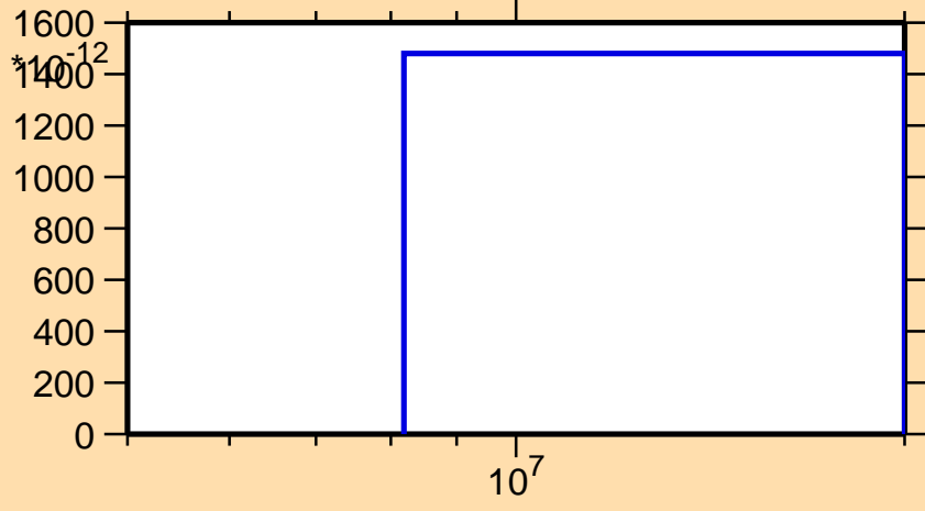
\sigma vs. E for ^{192}\text{Pb}(\text{mt } 45)
