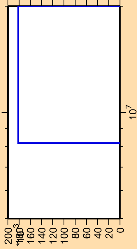
\Delta\sigma/\sigma vs. E for ^{192}\text{Pb} (mt 34)
