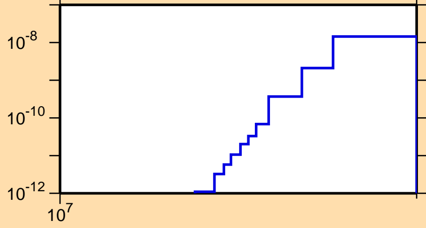
\sigma vs. E for ^{193}\text{Pb}(n,\text{pd})
