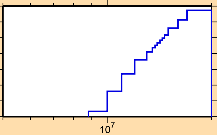
\sigma vs. E for ^{193}\text{Pb}(n,\text{He3})
