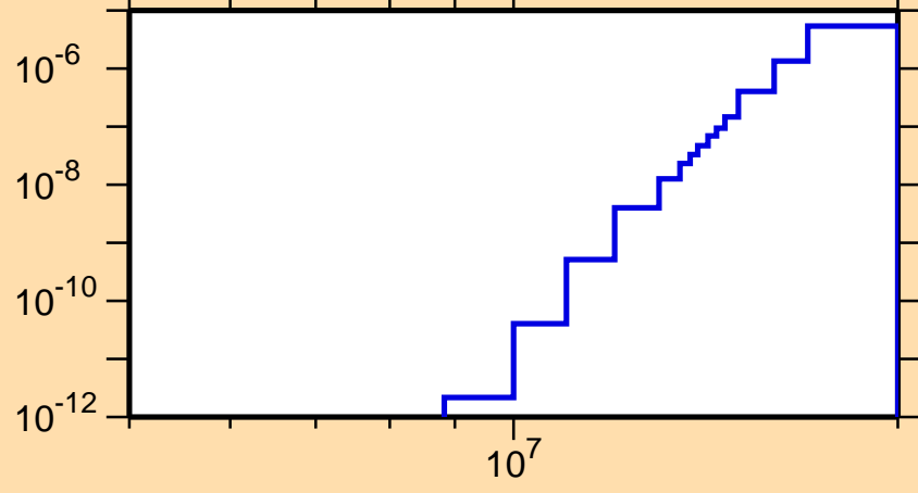
\sigma vs. E for ^{193}\text{Pb}(n,\text{He3})
