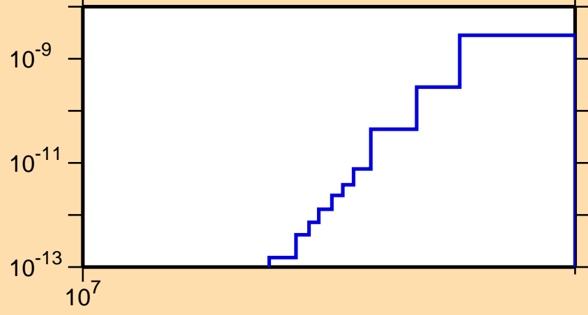
\sigma vs. E for ^{193}\text{Pb}(\text{mt } 45)
