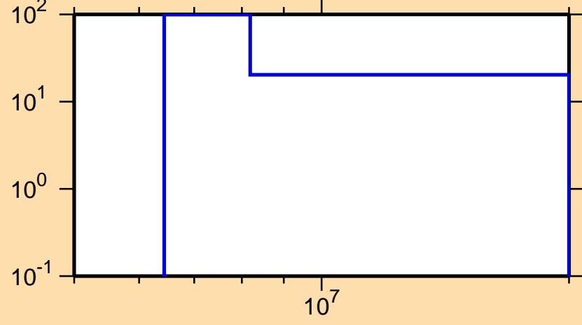
\Delta\sigma/\sigma vs. E for ^{193}\text{Pb}(n,2n)
