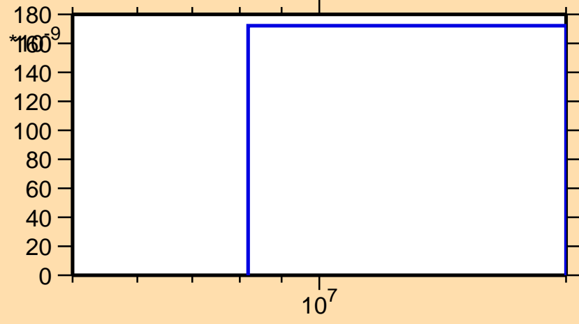
\sigma vs. E for ^{193}\text{Pb}(n,\text{He3})
