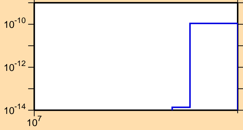
\sigma vs. E for ^{193}\text{Pb}(n,nt)
