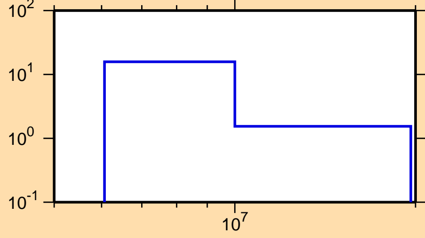
\Delta\sigma/\sigma vs. E for ^{193}\text{Pb}(n,\text{tot.})
