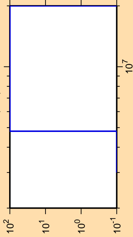
\Delta\sigma/\sigma vs. E for ^{193}\text{Pb}(n,d)
