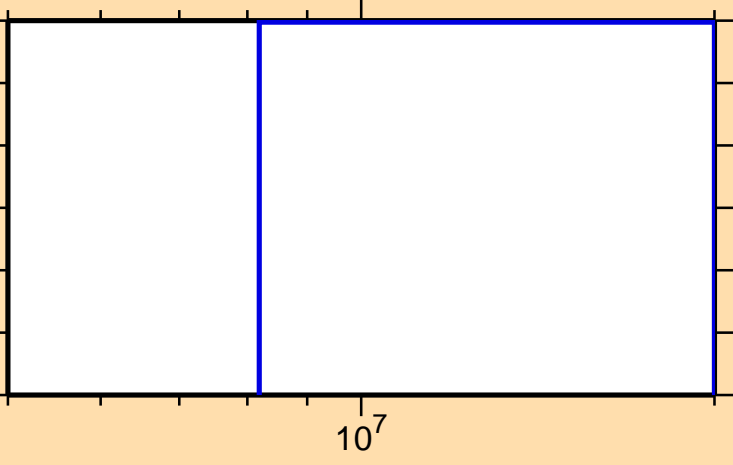
\sigma vs. E for ^{193}\text{Pb}(n,\text{He3})
