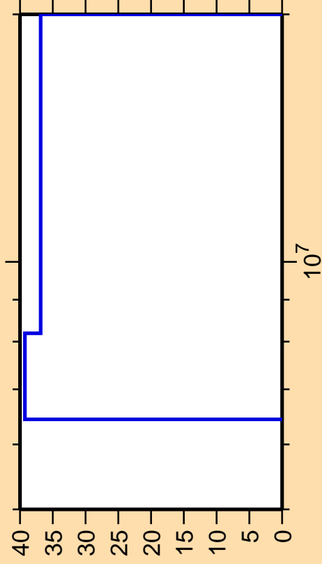
\Delta\sigma/\sigma vs. E for ^{193}\text{Pb}(n,\gamma)
