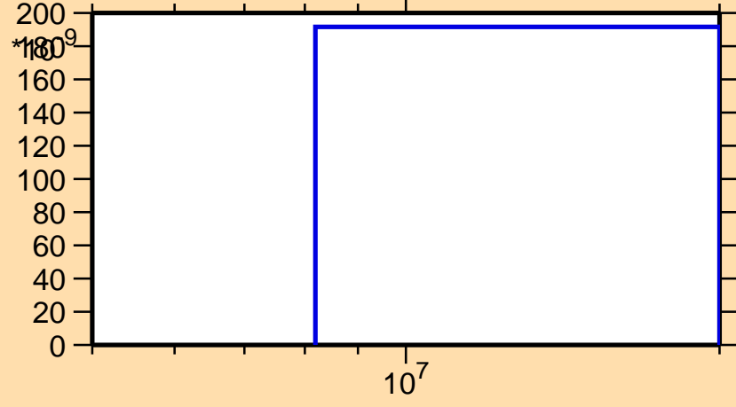
\sigma vs. E for ^{193}\text{Pb}(n,2n\alpha)
