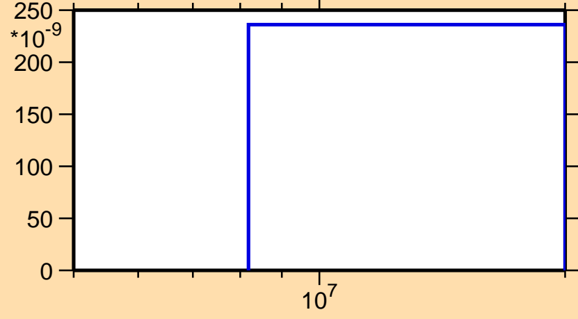
\sigma vs. E for ^{193}\text{Pb}(n,3n)
