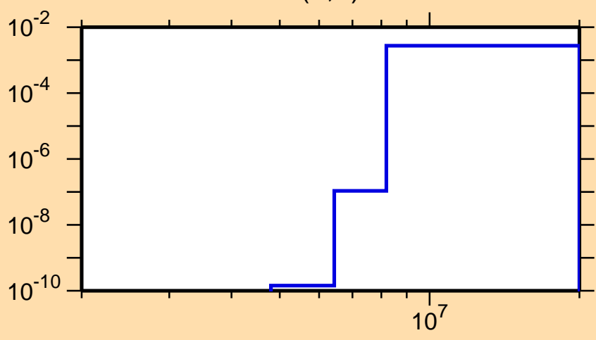
\sigma vs. E for ^{193}\text{Pb}(n,d)
