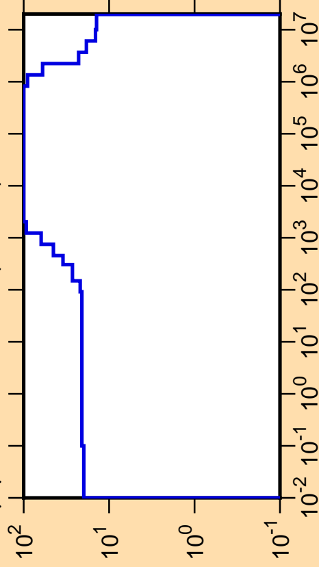
\Delta\mu/\mu vs. E for ^{195}\text{Pb}(\text{mt251})
