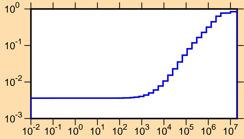
\mu vs. E for ^{195}\text{Pb}(\text{mt251})
