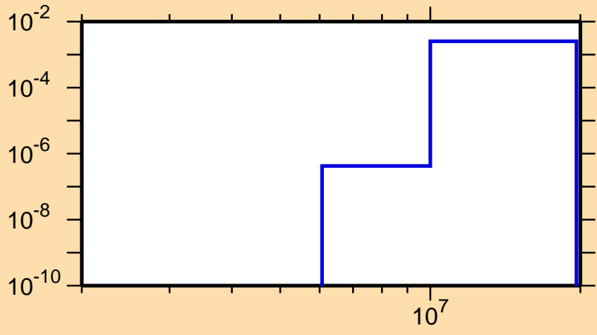
\sigma vs. E for ^{195}\text{Pb}(n,d)
