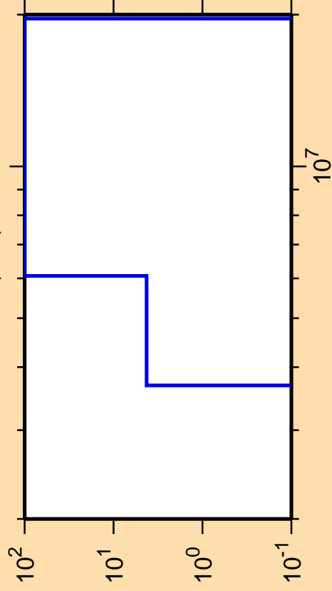
\Delta\sigma/\sigma vs. E for ^{195}\text{Pb}(n,d)
