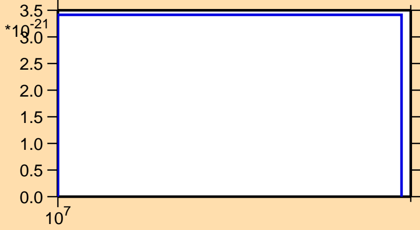
\sigma vs. E for ^{195}\text{Pb} (mt 11)
