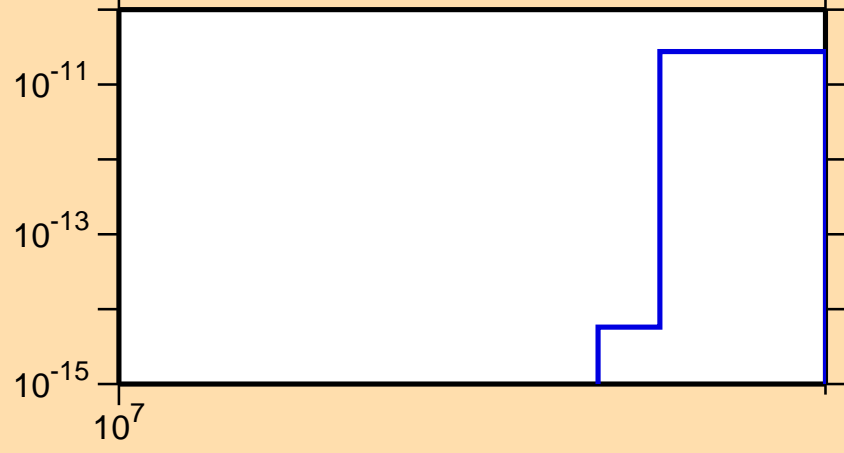
\sigma vs. E for ^{195}\text{Pb}(n,nt)
