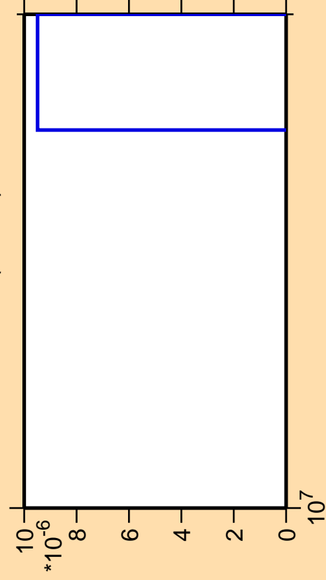
\Delta\sigma/\sigma vs. E for ^{195}\text{Pb}(\text{mt } 11)
