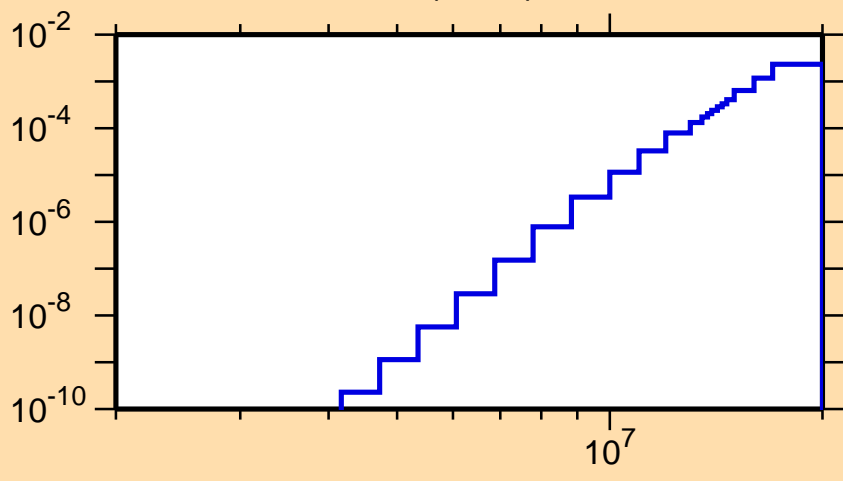
\sigma vs. E for ^{195}\text{Pb}(n,n\alpha)
