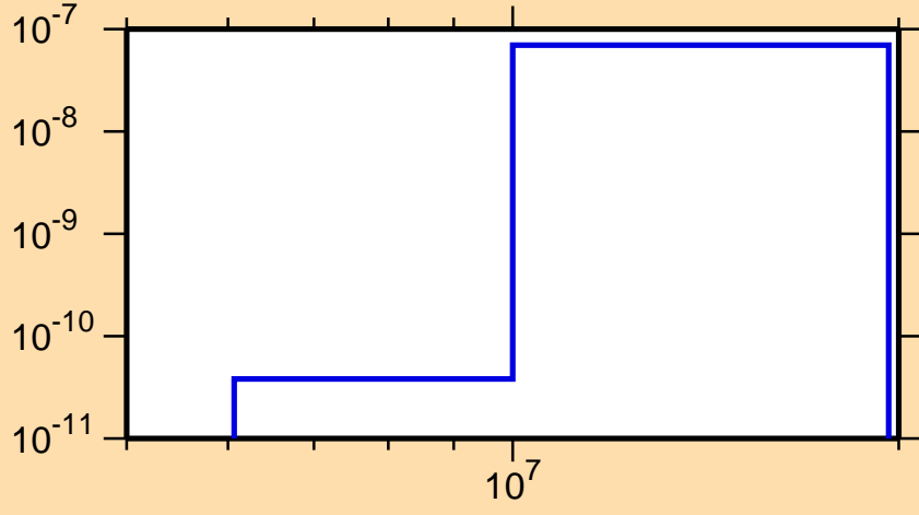
\sigma vs. E for ^{195}\text{Pb}(n,p\alpha)
