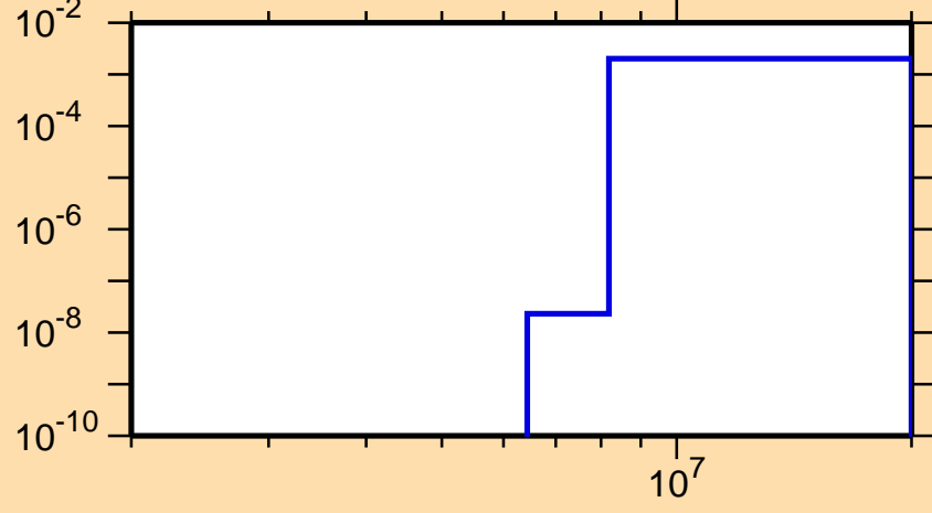
\sigma vs. E for ^{195}\text{Pb}(n,d)
