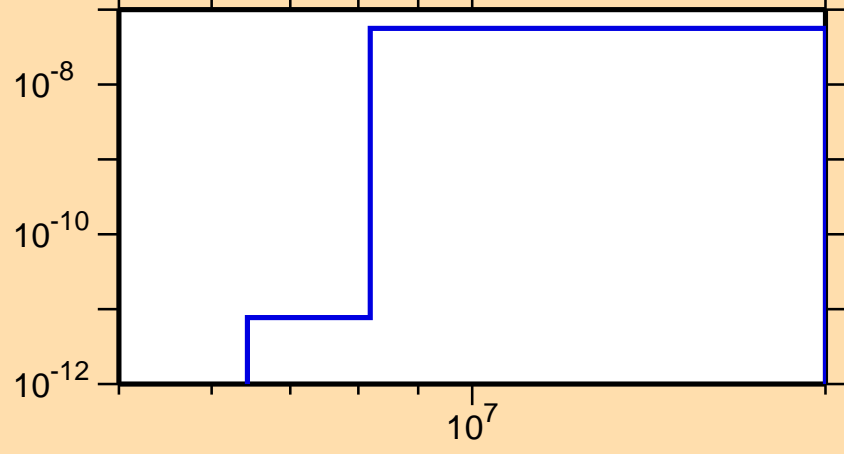
\sigma vs. E for ^{195}\text{Pb}(n,p\alpha)
