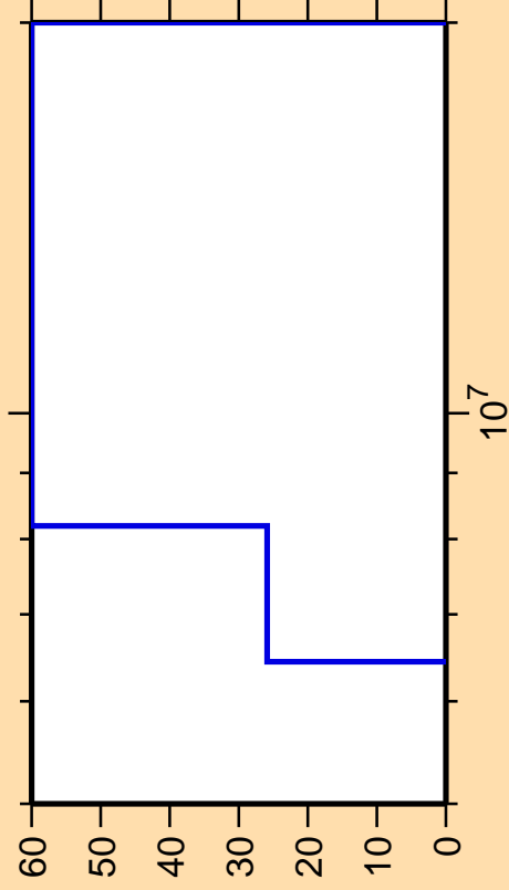
\Delta\sigma/\sigma vs. E for ^{195}\text{Pb}(n,p\alpha)
