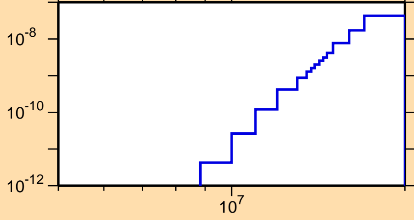
\sigma vs. E for ^{197}\text{Pb}(n,p\alpha)
