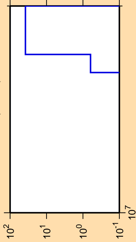
\Delta\sigma/\sigma vs. E for ^{197}\text{Pb} (mt 34)
