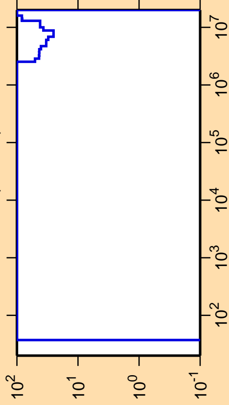
\Delta\sigma/\sigma vs. E for ^{197}\text{Pb}(n,\text{inel.})
