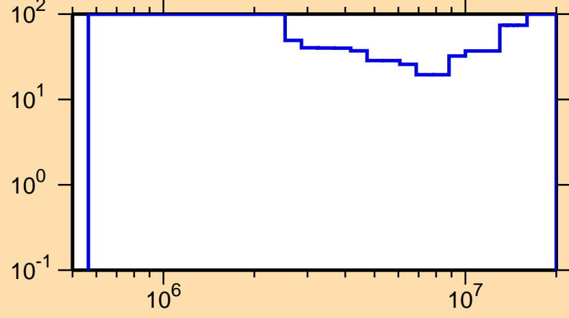
\Delta\sigma/\sigma vs. E for ^{197}\text{Pb}(n,ncont.)
