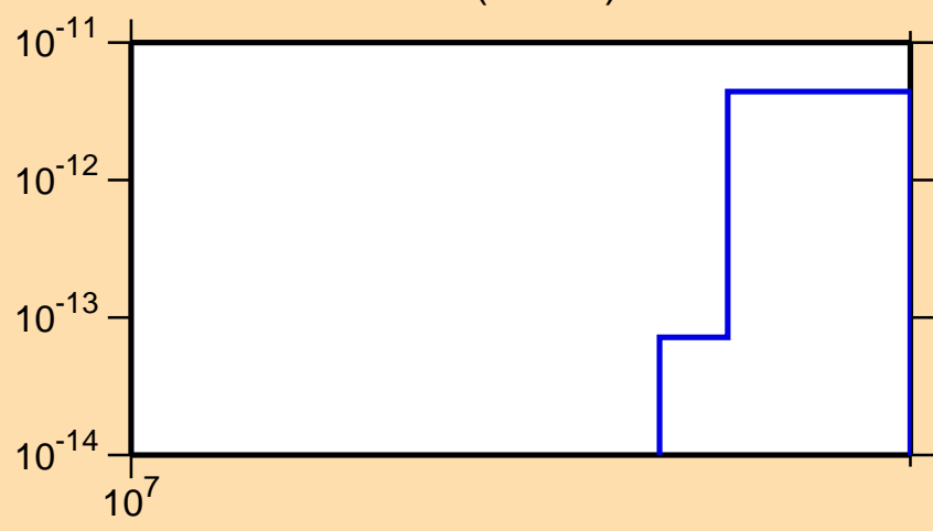
\sigma vs. E for ^{197}\text{Pb} (mt 34)
