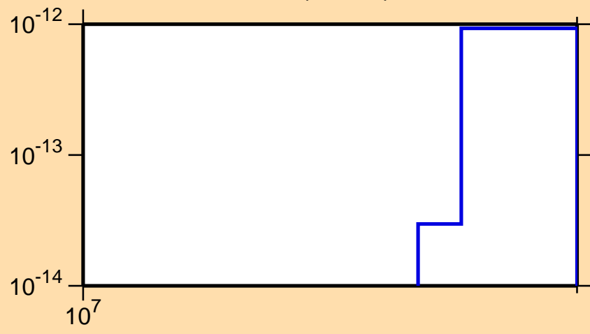
\sigma vs. E for ^{197}\text{Pb} (mt 45)
