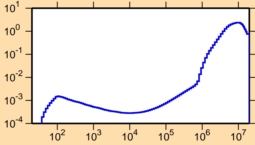
\sigma vs. E for ^{197}\text{Pb}(n,\text{inel.})
