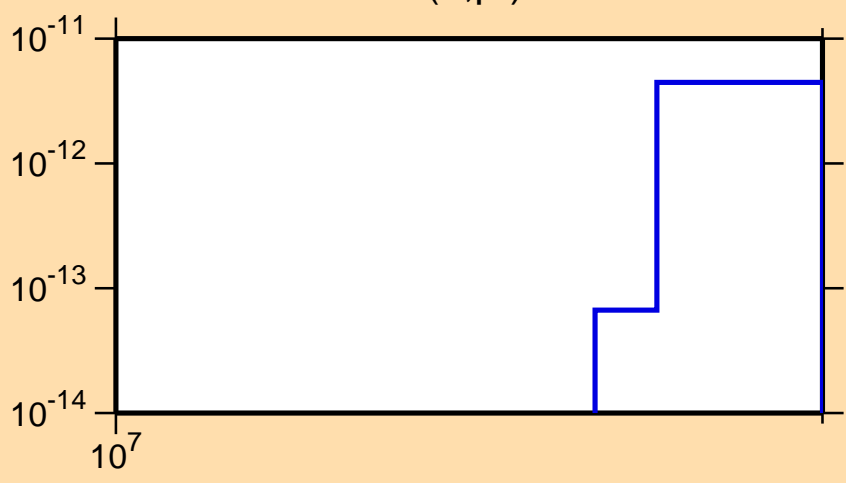
\sigma vs. E for ^{197}\text{Pb}(n,\text{pt})
