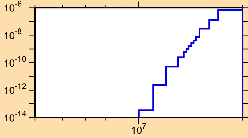
\sigma vs. E for ^{197}\text{Pb}(n,2n\alpha)
