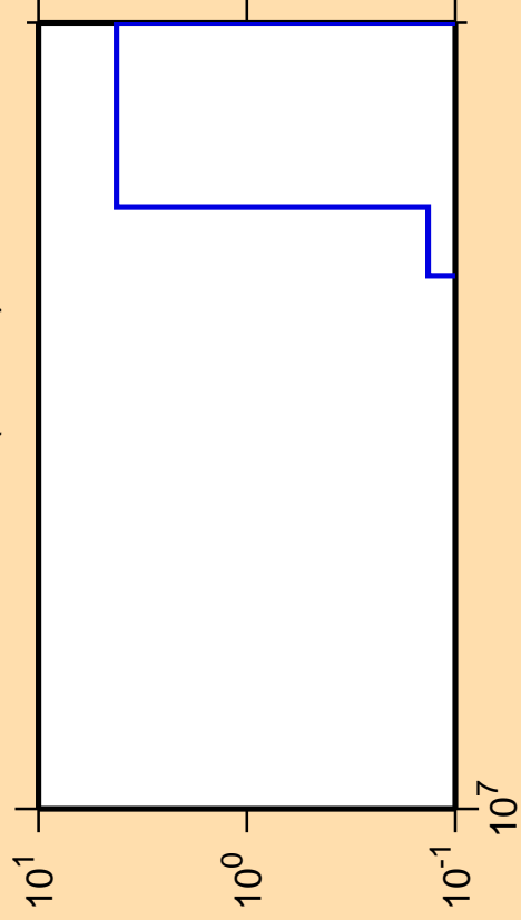
\Delta\sigma/\sigma vs. E for ^{197}\text{Pb} (mt 45)
