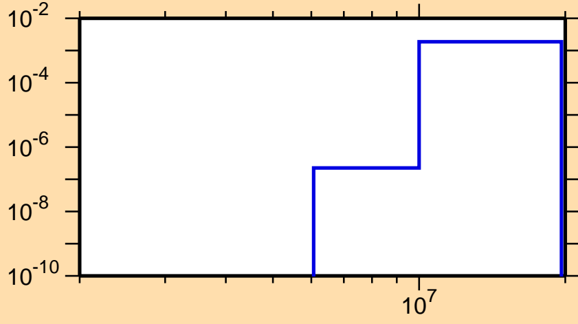
\sigma vs. E for ^{197}\text{Pb}(n,d)
