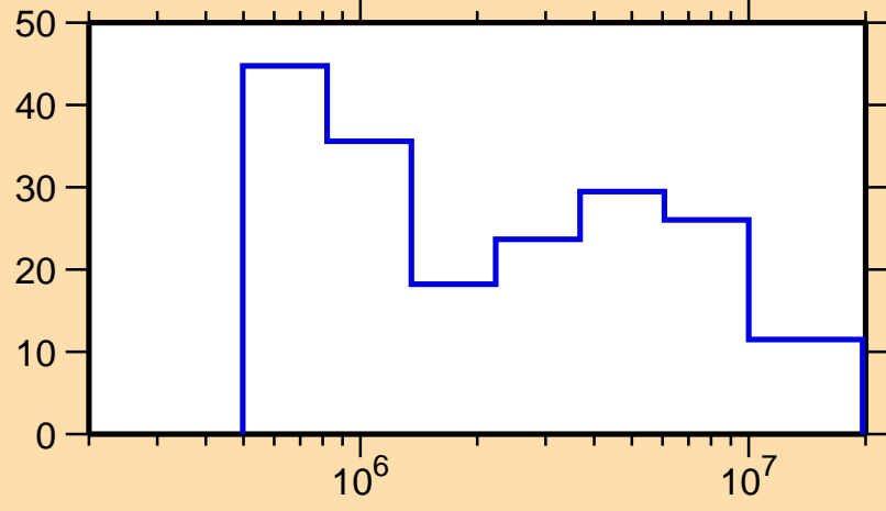
\Delta\sigma/\sigma vs. E for ^{197}\text{Pb}(n, el.)
