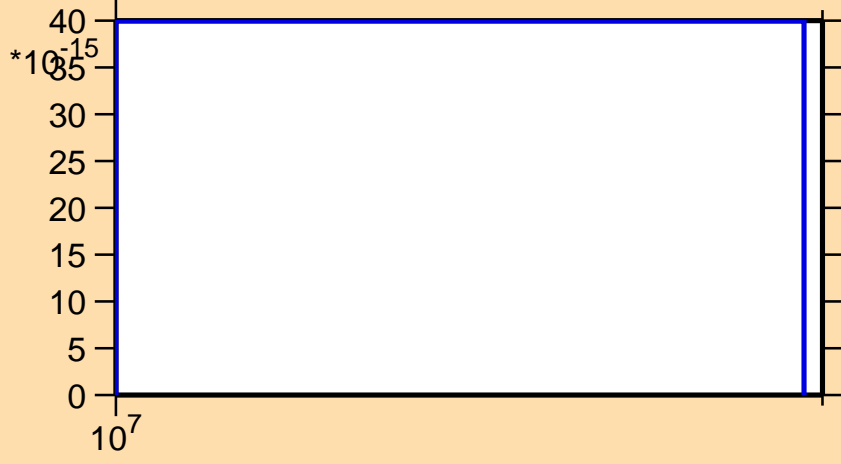
\sigma vs. E for ^{197}\text{Pb} (mt 34)
