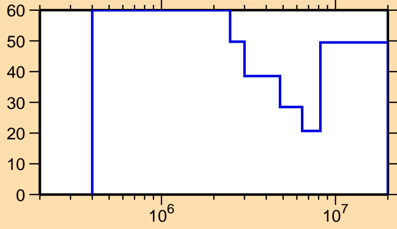
\Delta\sigma/\sigma vs. E for ^{197}\text{Pb}(n,n\text{cont.})
