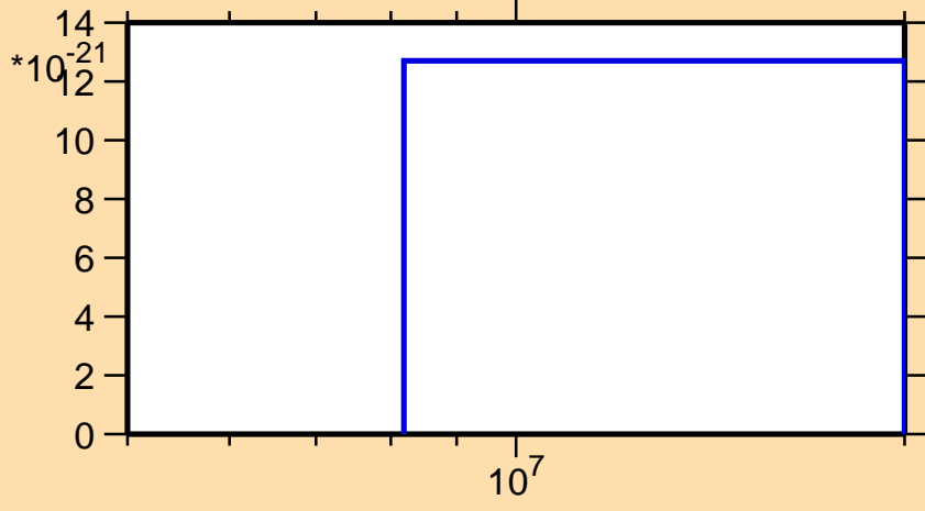
\sigma vs. E for ^{197}\text{Pb}(\text{mt } 11)
