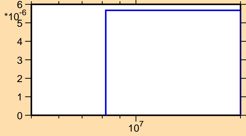
\sigma vs. E for ^{197}\text{Pb}(n,3n)
