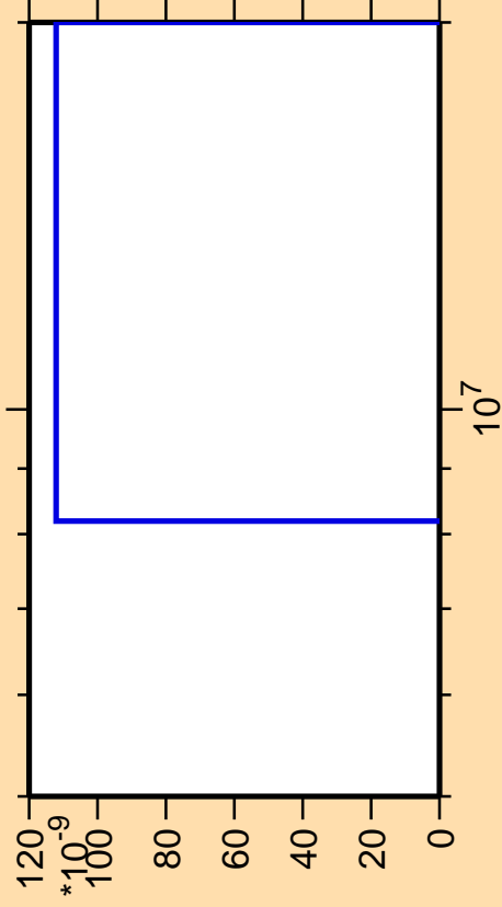
\Delta\sigma/\sigma vs. E for ^{197}\text{Pb}(\text{mt } 11)
