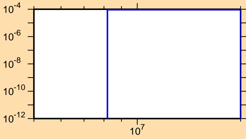
\sigma vs. E for ^{197}\text{Pb}(n,t)
