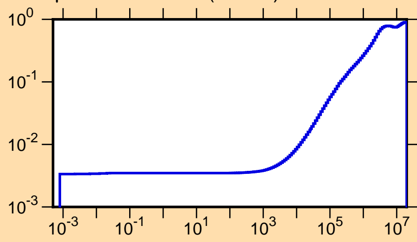
\mu vs. E for ^{201}\text{Pb}(\text{mt251})
