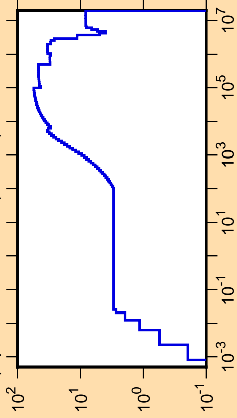
\Delta\mu/\mu vs. E for ^{201}\text{Pb}(\text{mt251})
