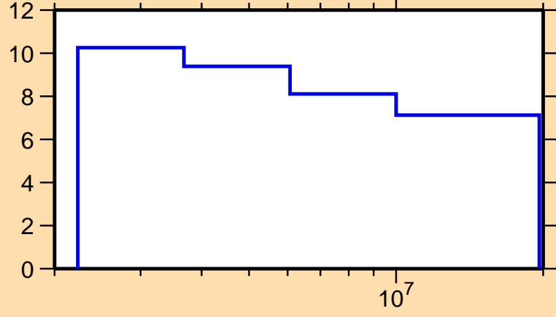
\Delta\sigma/\sigma vs. E for ^{201}\text{Pb}(n,n\text{onel.})
