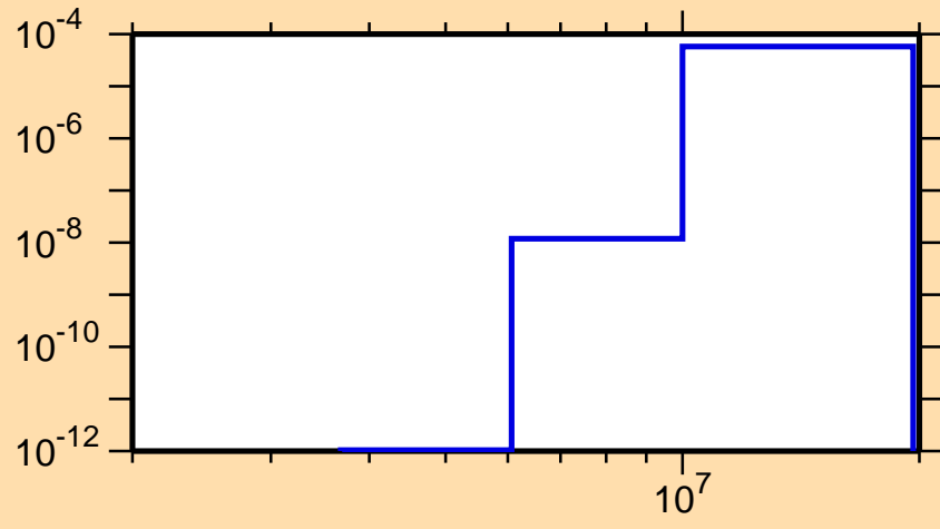
\sigma vs. E for ^{201}\text{Pb}(n,n\alpha)
