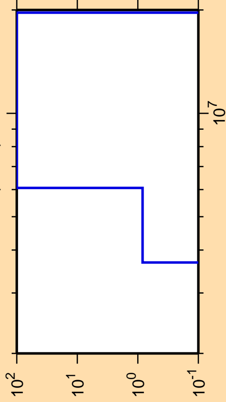
\Delta\sigma/\sigma vs. E for ^{201}\text{Pb}(n,n\alpha)
