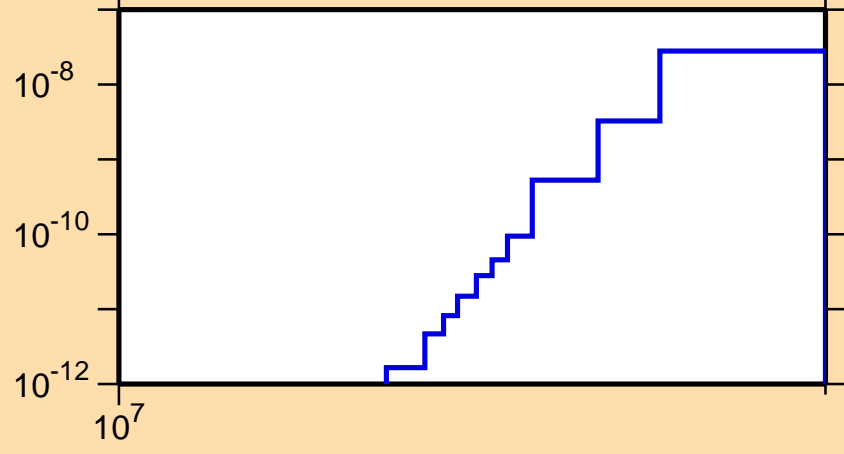
\sigma vs. E for ^{201}\text{Pb}(n,\text{He3})
