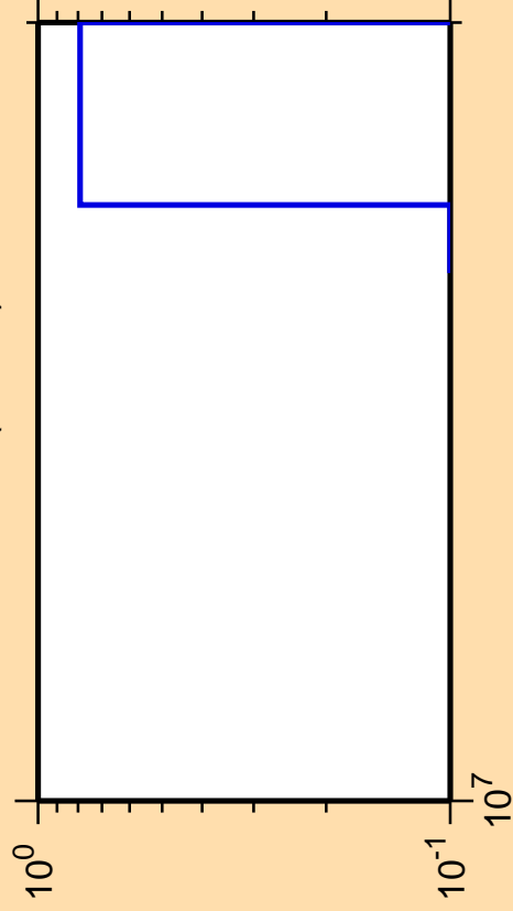
\Delta\sigma/\sigma vs. E for ^{201}\text{Pb} (mt 34)
