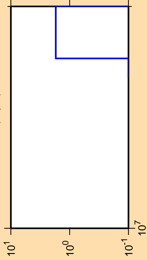
\Delta\sigma/\sigma vs. E for ^{201}\text{Pb}(n,\text{pd})
