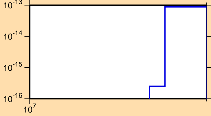
\sigma vs. E for ^{201}\text{Pb} (mt 34)
