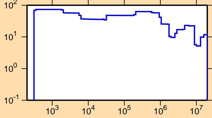
\Delta\sigma/\sigma vs. E for ^{201}\text{Pb}(n,\text{el.})
