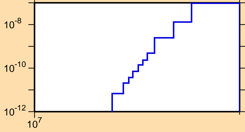
\sigma vs. E for ^{201}\text{Pb}(n,2n\alpha)
