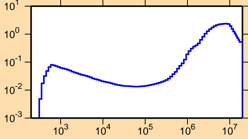
\sigma vs. E for ^{201}\text{Pb}(n,\text{inel.})
