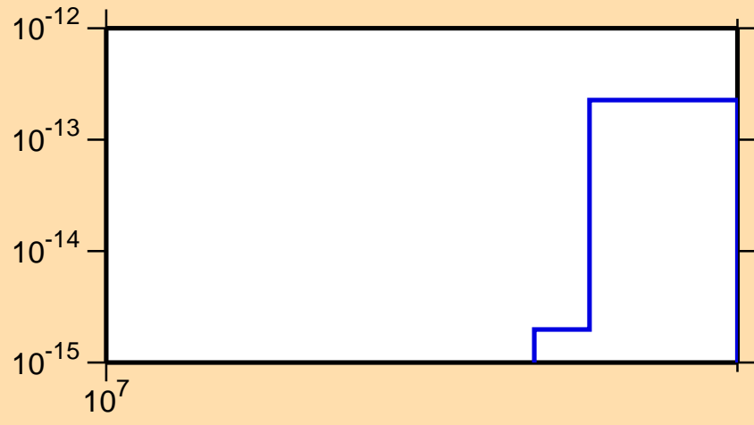
\sigma vs. E for ^{201}\text{Pb}(n,\text{pd})
