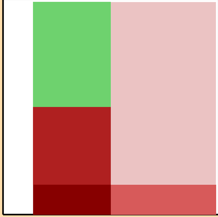
\Delta\sigma/\sigma vs. E for ^{201}\text{Pb}(n,2n)
