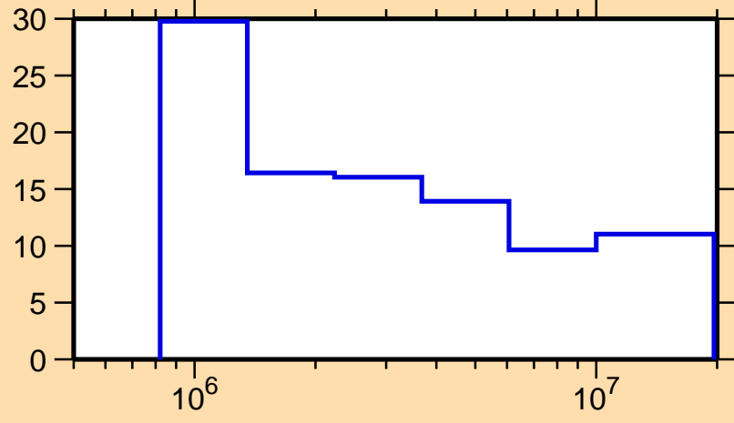
\Delta\sigma/\sigma vs. E for ^{201}\text{Pb}(n,n\text{nonel.})
