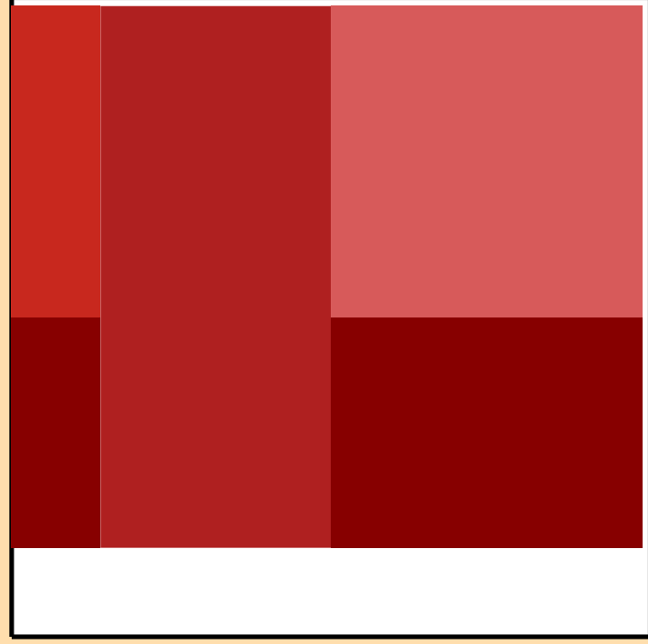
\Delta\sigma/\sigma vs. E for ^{201}\text{Pb}(n,\text{tot.})
