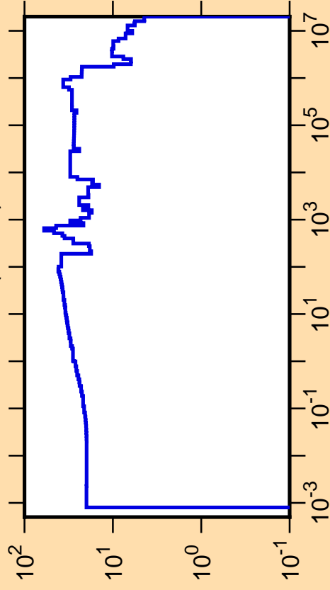
\Delta\sigma/\sigma vs. E for ^{202}\text{Pb}(n,\text{tot.})
