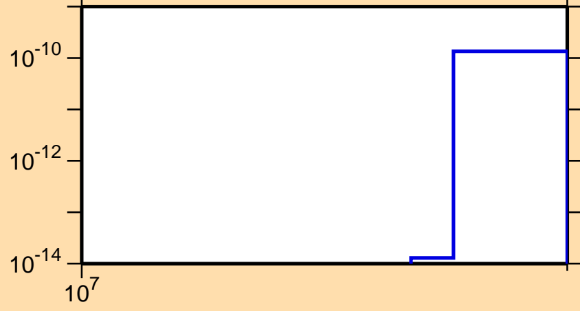
\sigma vs. E for ^{202}\text{Pb}(n,nt)
