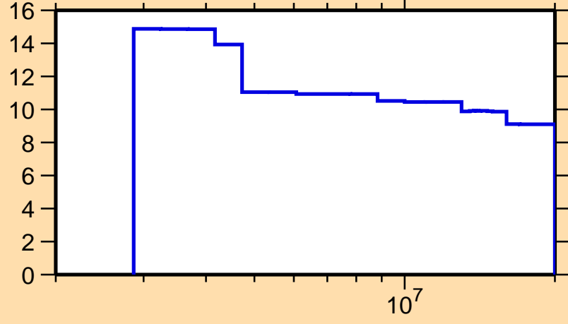
\Delta\sigma/\sigma vs. E for ^{202}\text{Pb}(n,n\text{nonel.})
