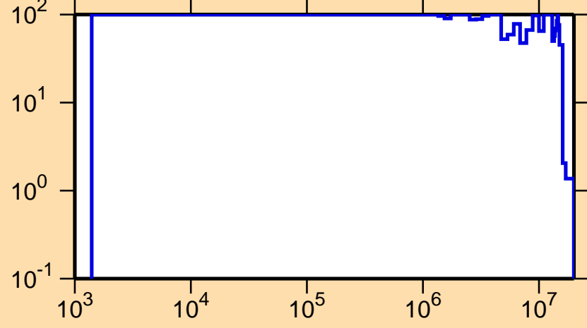
\Delta\sigma/\sigma vs. E for ^{202}\text{Pb}(n,n_1)
