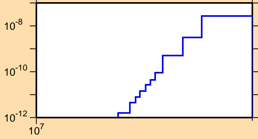
\sigma vs. E for ^{202}\text{Pb}(n,\text{He3})
