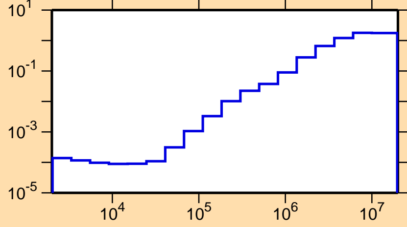
\sigma vs. E for ^{202}\text{Pb}(n,\text{inel.})
