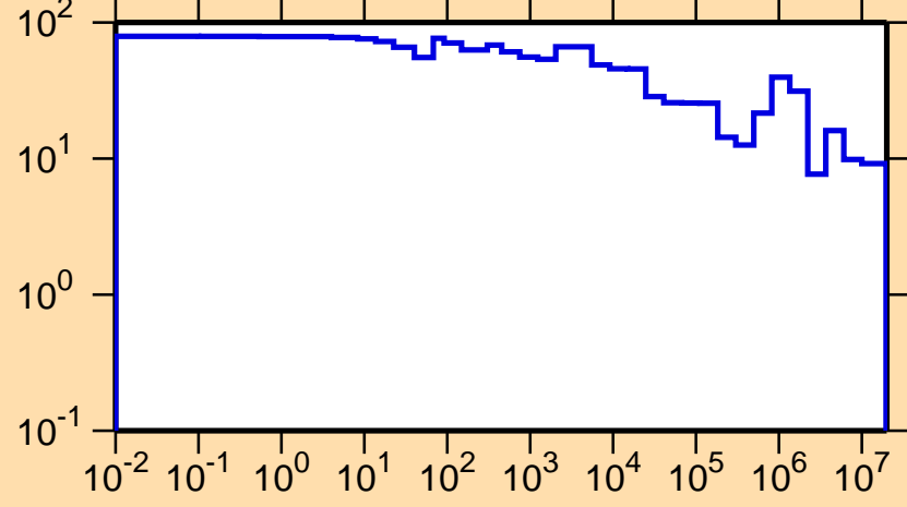
\Delta\sigma/\sigma vs. E for ^{202}\text{Pb}(n,\text{el.})
