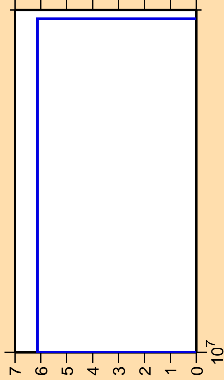
\Delta\sigma/\sigma vs. E for ^{202}\text{Pb}(n,p\alpha)
