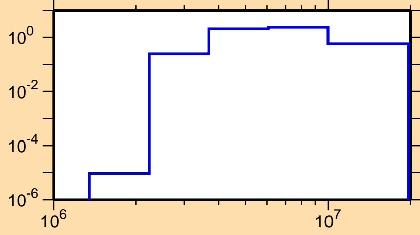
\sigma vs. E for ^{203}\text{Pb}(n,n\text{cont.})
