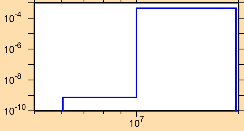
\sigma vs. E for ^{203}\text{Pb}(n,d)
