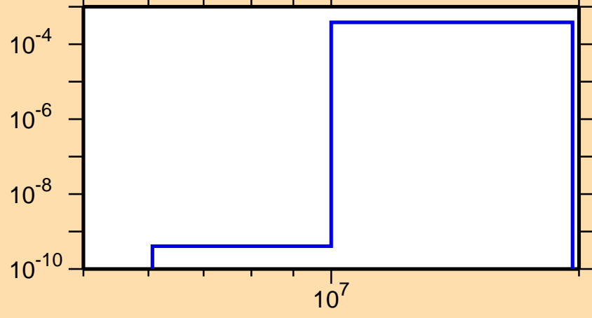
\sigma vs. E for ^{203}\text{Pb}(n,np)
