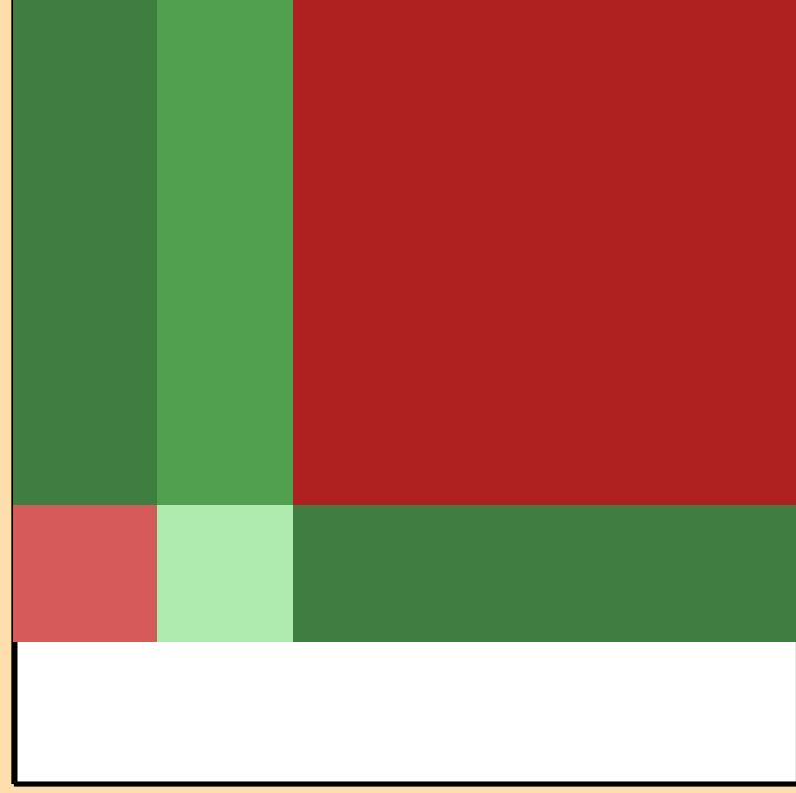
\Delta\sigma/\sigma vs. E for ^{203}\text{Pb}(n,\text{el.})
