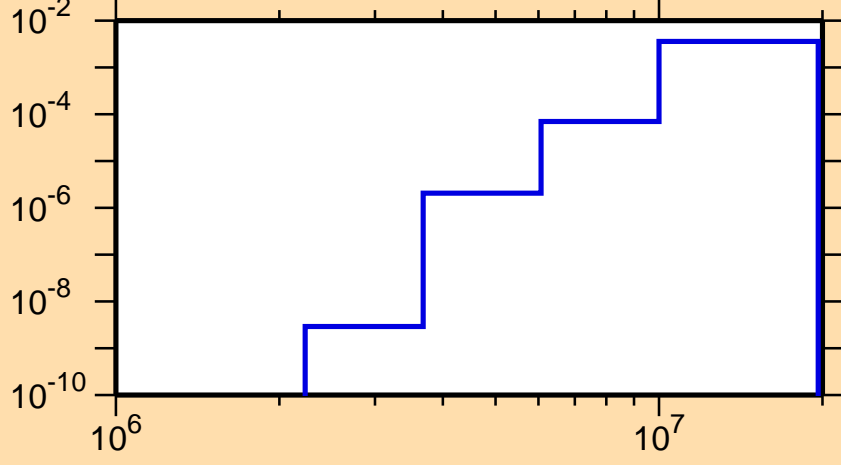
\sigma vs. E for ^{204}\text{Pb}(n,p)
