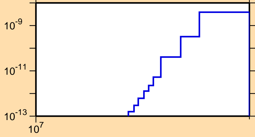
\sigma vs. E for ^{204}\text{Pb}(n,\text{He3})
