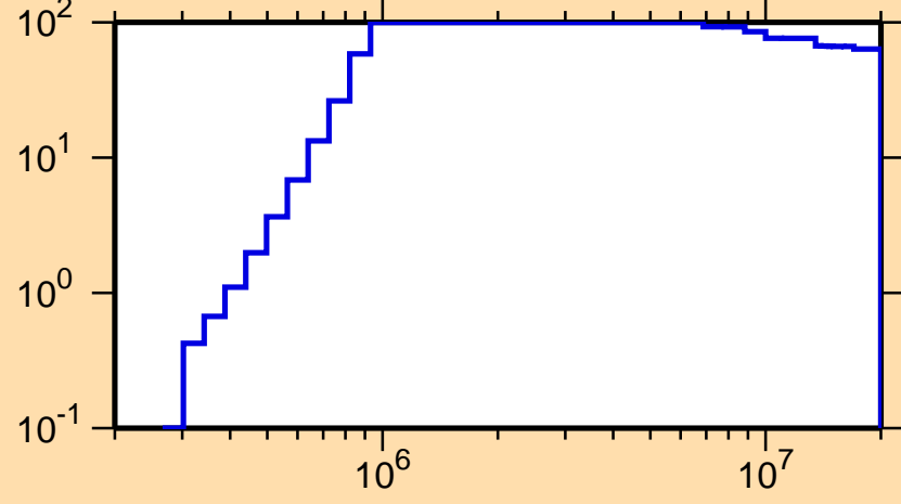
\Delta\sigma/\sigma vs. E for ^{204}\text{Pb}(n,p)
