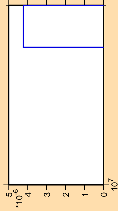
\Delta\sigma/\sigma vs. E for ^{204}\text{Pb} (mt 42)
