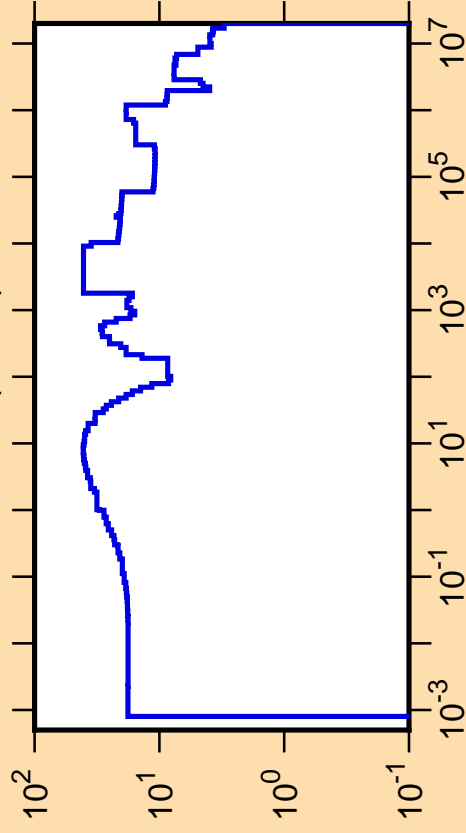
\Delta\sigma/\sigma vs. E for ^{204}\text{Pb}(n,\text{tot.})
