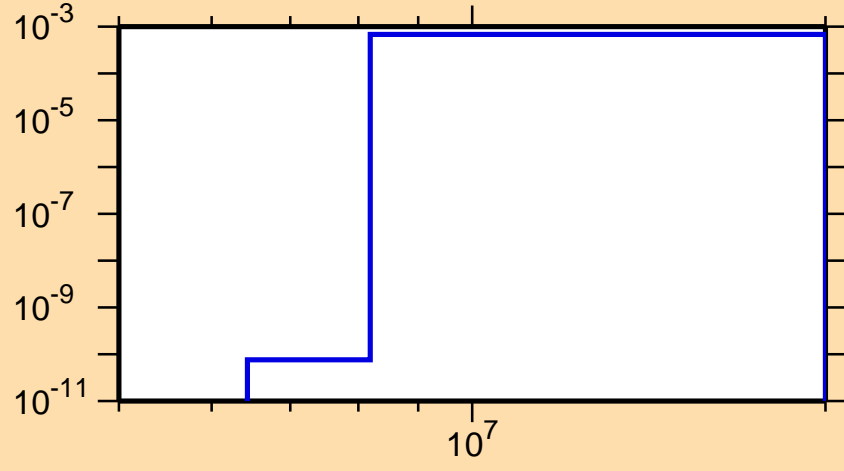
\sigma vs. E for ^{204}\text{Pb}(n,d)
