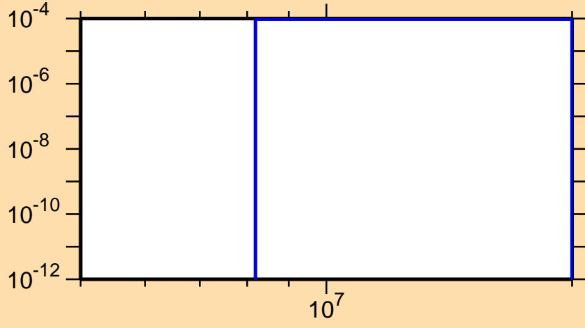
\sigma vs. E for ^{204}\text{Pb}(n,t)
