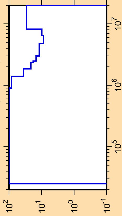
\Delta\sigma/\sigma vs. E for ^{204}\text{Pb}(n,\text{ncont.})
