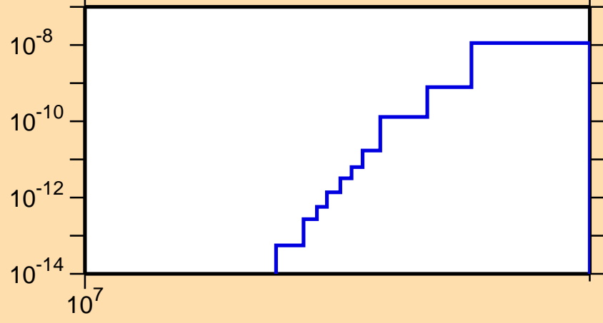
\sigma vs. E for ^{205}\text{Pb}(n,2n\alpha)
