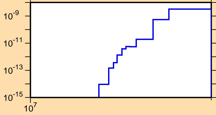
\sigma vs. E for ^{205}\text{Pb}(n,p\alpha)
