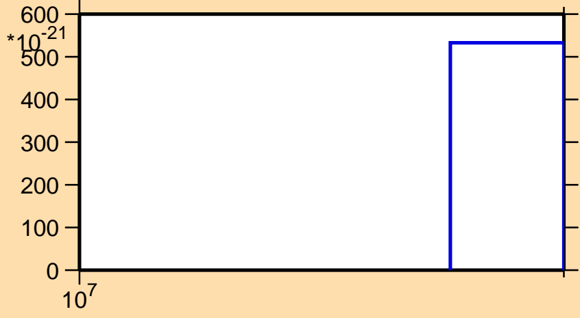
\sigma vs. E for ^{205}\text{Pb}(\text{mt } 11)
