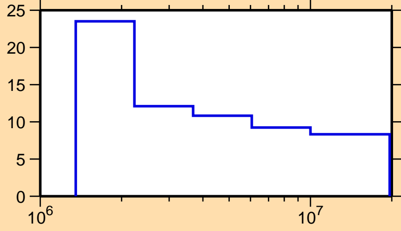
\Delta\sigma/\sigma vs. E for ^{205}\text{Pb}(n,n\text{onel.})
