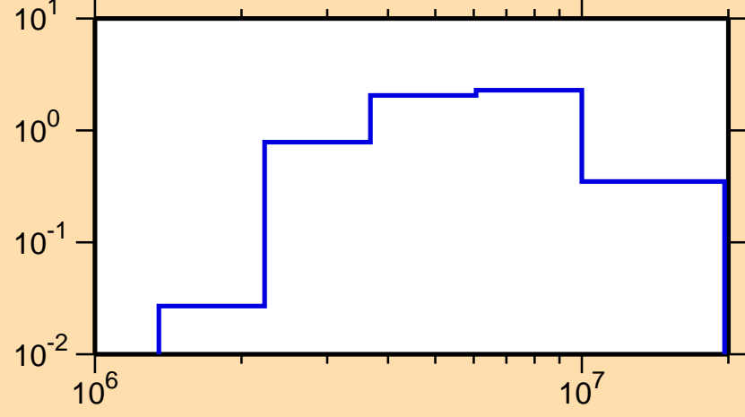
\sigma vs. E for ^{205}\text{Pb}(n,n\text{cont.})
