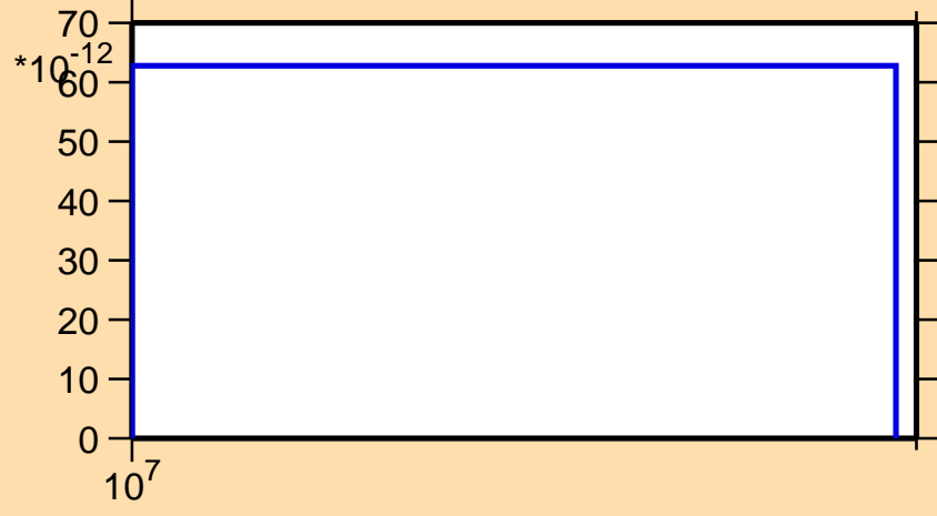
\sigma vs. E for ^{205}\text{Pb}(n,p\alpha)
