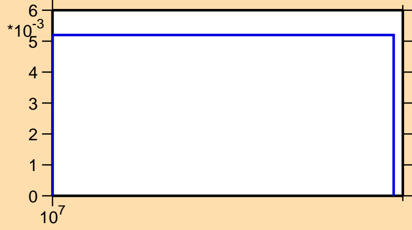
\sigma vs. E for ^{205}\text{Pb}(n,3n)
