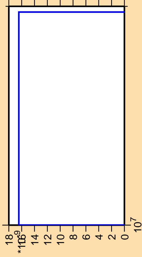
\Delta\sigma/\sigma vs. E for ^{205}\text{Pb} (mt 11)
