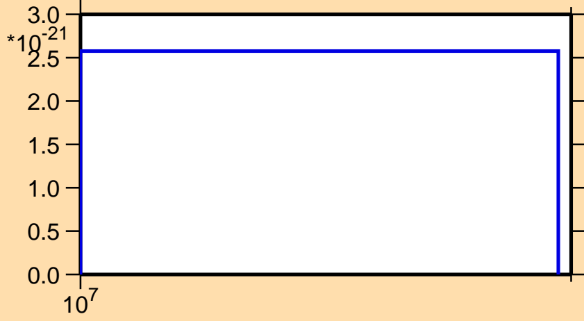
\sigma vs. E for ^{205}\text{Pb} (mt 11)
