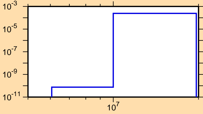
\sigma vs. E for ^{205}\text{Pb}(n,d)
