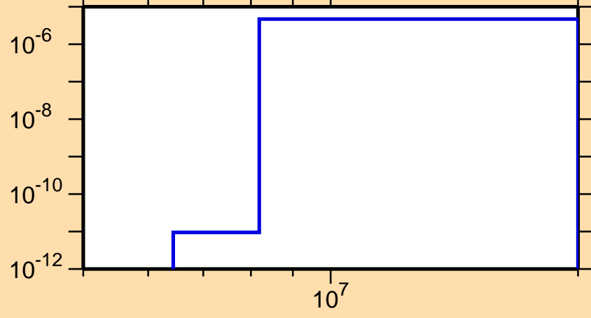
\sigma vs. E for ^{205}\text{Pb}(n,n\alpha)
