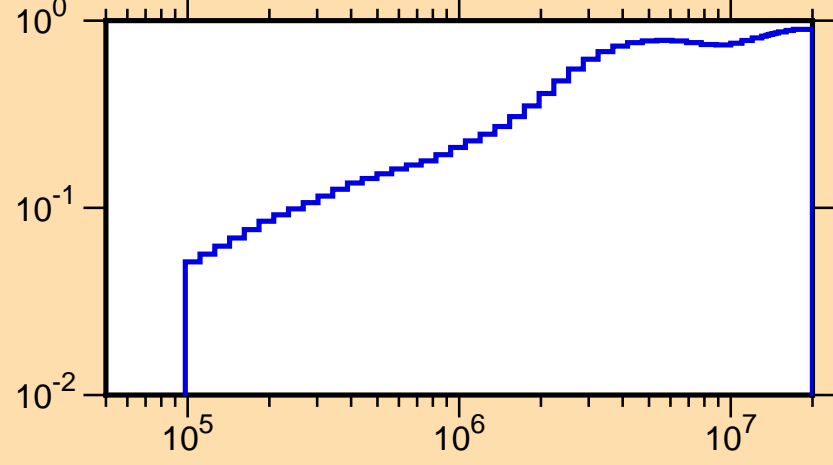
\mu vs. E for ^{206}\text{Pb}(\text{mt251})
