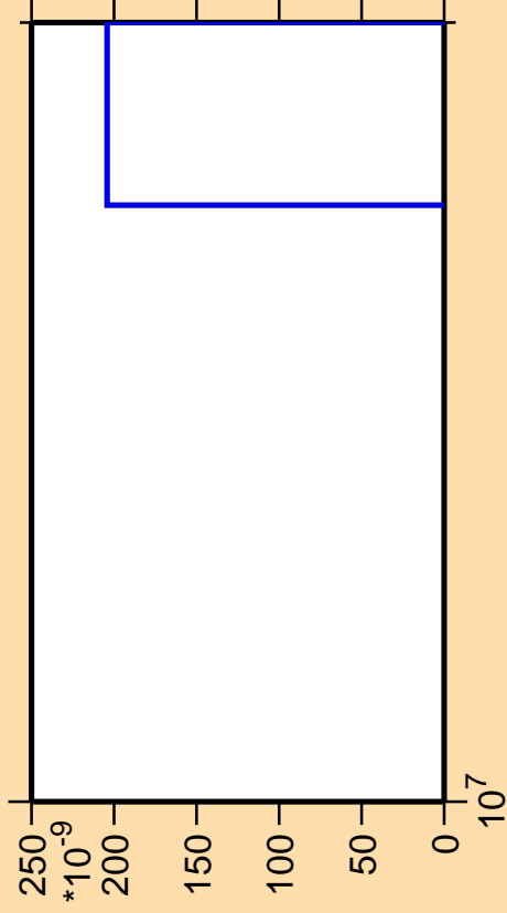
\Delta\sigma/\sigma vs. E for ^{206}\text{Pb} (mt 11)
