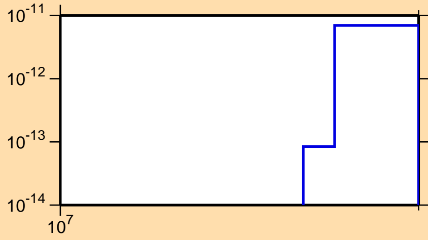
\sigma vs. E for ^{206}\text{Pb}(n,\text{He}3)
