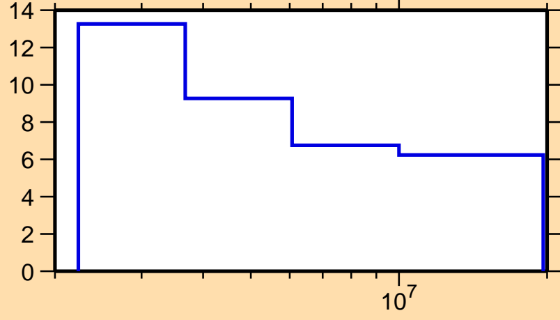
\Delta\sigma/\sigma vs. E for ^{206}\text{Pb}(n,n\text{nonel.})
