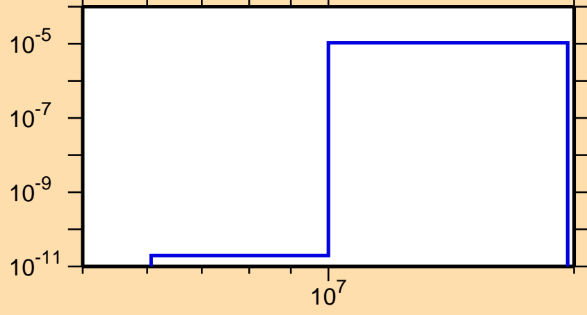
\sigma vs. E for ^{206}\text{Pb}(n,n\alpha)
