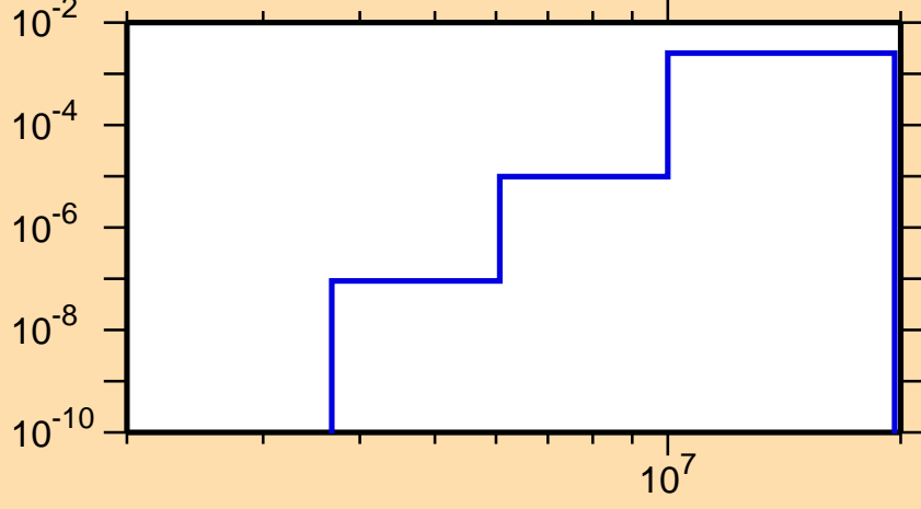
\sigma vs. E for ^{206}\text{Pb}(n,p)
