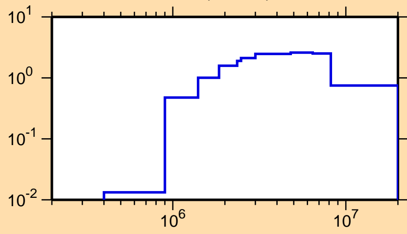
\sigma vs. E for ^{206}\text{Pb}(n,\text{inel.})
