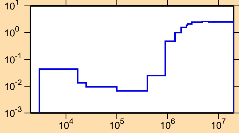
\sigma vs. E for ^{206}\text{Pb}(n,\text{nonel.})
