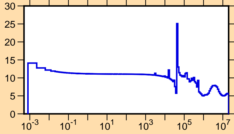
\sigma vs. E for ^{207}\text{Pb}(n,\text{tot.})
