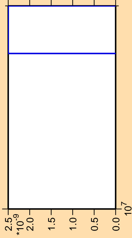
\Delta\sigma/\sigma vs. E for ^{207}\text{Pb} (mt 11)
