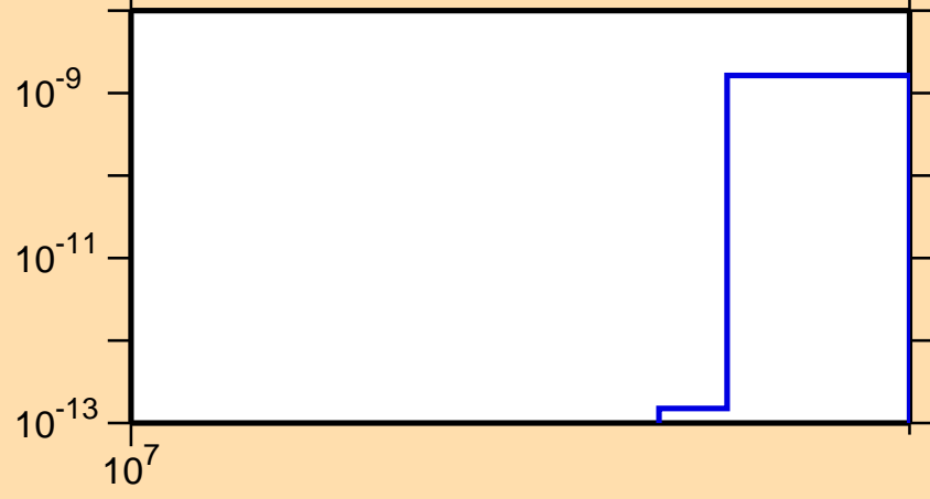
\sigma vs. E for ^{207}\text{Pb}(n,2np)
