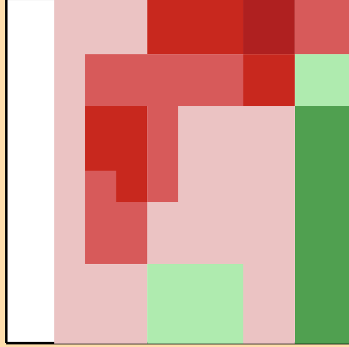
\Delta\sigma/\sigma vs. E for ^{207}\text{Pb}(n,2n)
