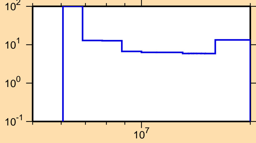
\Delta\sigma/\sigma vs. E for ^{207}\text{Pb}(n,2n)
