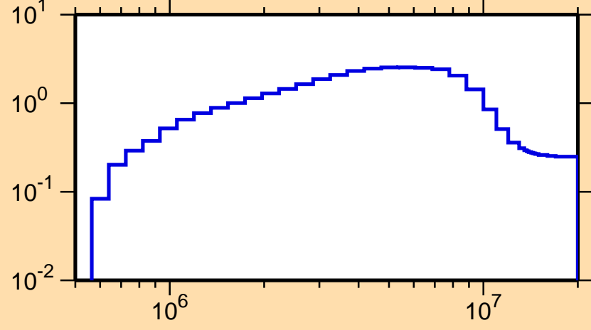
\sigma vs. E for ^{207}\text{Pb}(n,\text{inel.})
