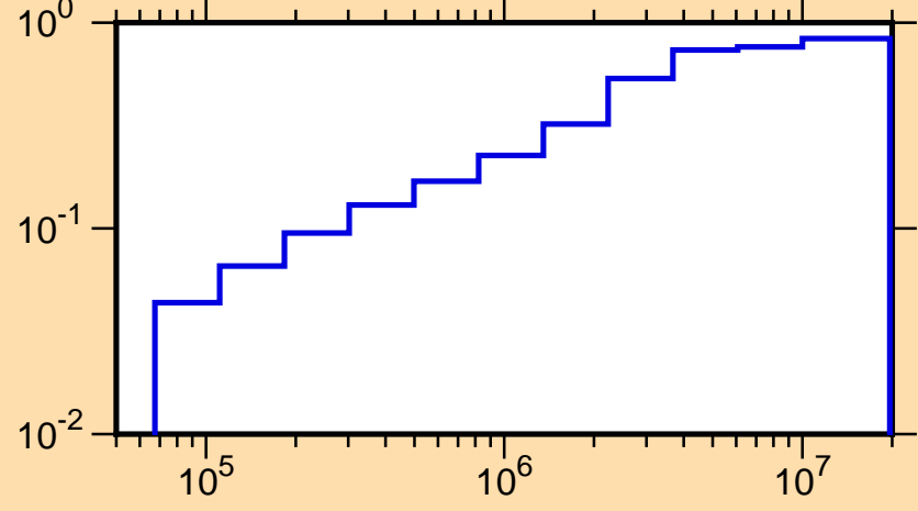
\mu vs. E for ^{207}\text{Pb}(\text{mt251})
