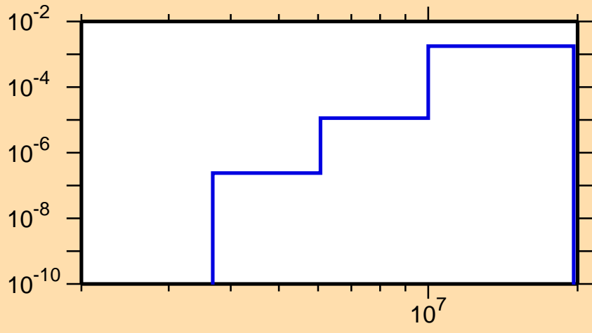
\sigma vs. E for ^{207}\text{Pb}(n,p)
