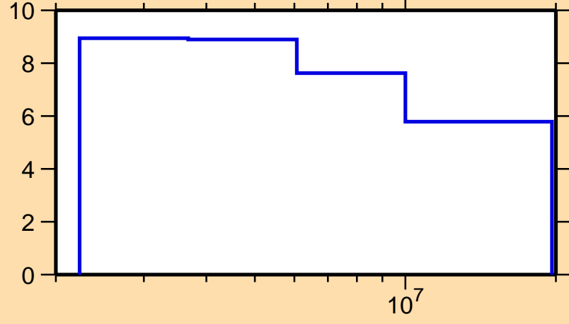
\Delta\sigma/\sigma vs. E for ^{207}\text{Pb}(n,n\text{nonel.})
