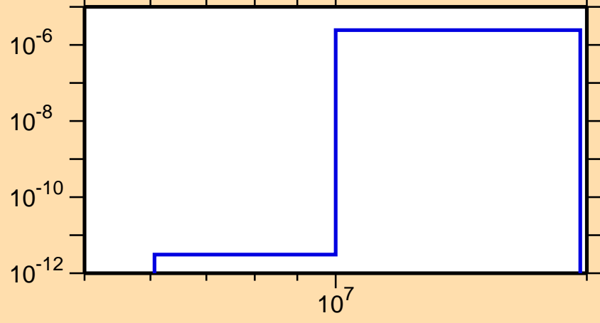
\sigma vs. E for ^{207}\text{Pb}(n,n\alpha)
