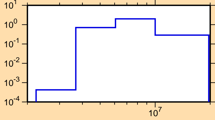
\sigma vs. E for ^{207}\text{Pb}(n,n\text{cont.})
