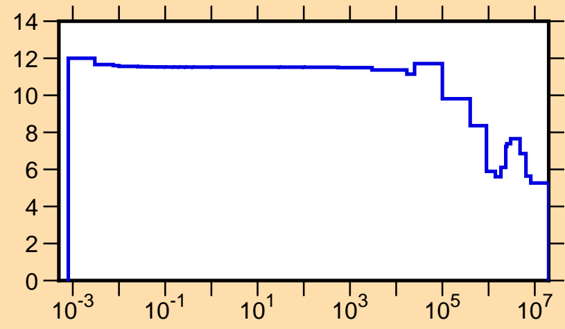
\sigma vs. E for ^{208}\text{Pb}(n,\text{tot.})
