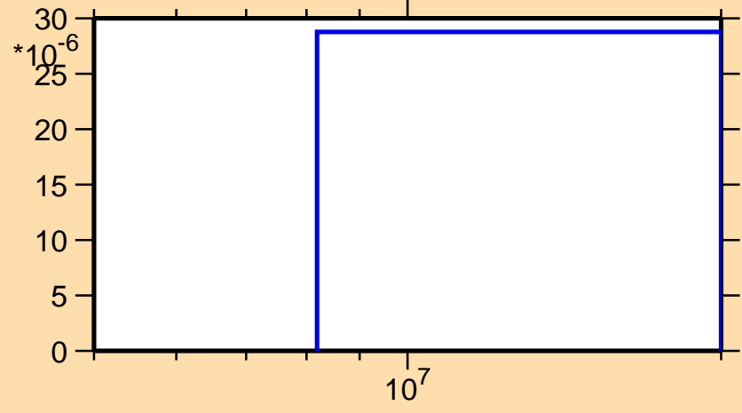
\sigma vs. E for ^{208}\text{Pb}(n,np)
