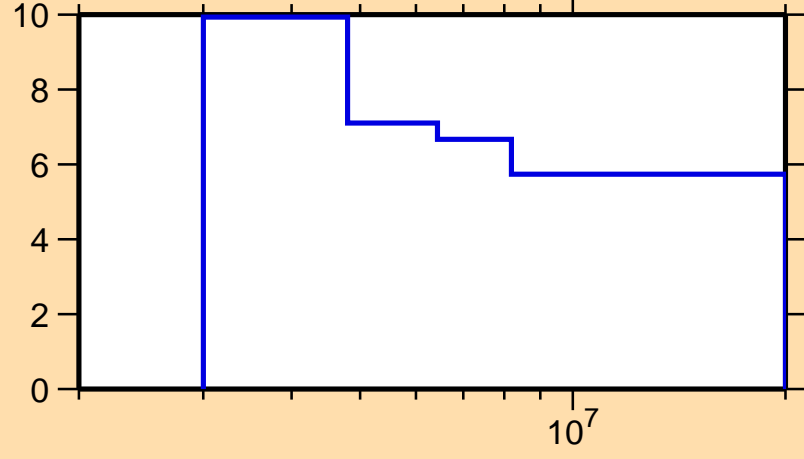
\Delta\sigma/\sigma vs. E for ^{208}\text{Pb}(n,n\text{nonel.})
