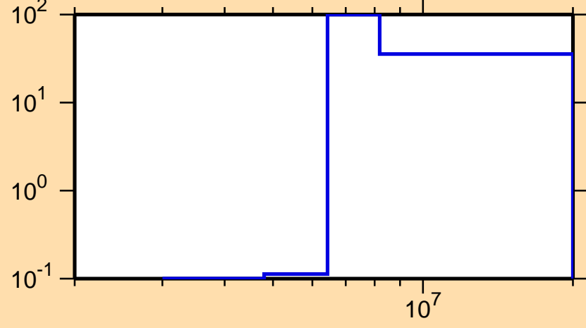
\Delta\sigma/\sigma vs. E for ^{208}\text{Pb}(n,p)
