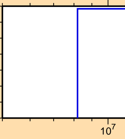
\sigma vs. E for ^{208}\text{Pb}(n,nt)
