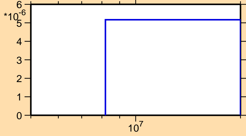
\sigma vs. E for ^{208}\text{Pb}(n,t)
