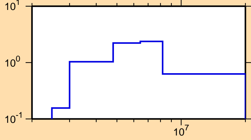
\sigma vs. E for ^{208}\text{Pb}(n,\text{inel.})
