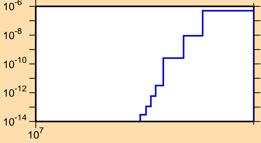
\sigma vs. E for ^{209}\text{Pb}(n,nt)
