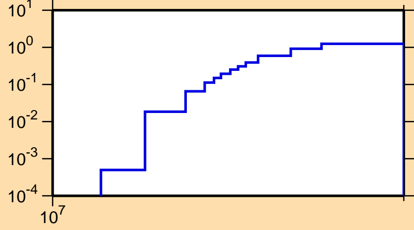
\sigma vs. E for ^{209}\text{Pb}(n,3n)
