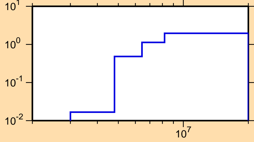
\sigma vs. E for ^{209}\text{Pb}(n,2n)
