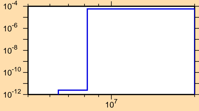
\sigma vs. E for ^{209}\text{Pb}(n,t)
