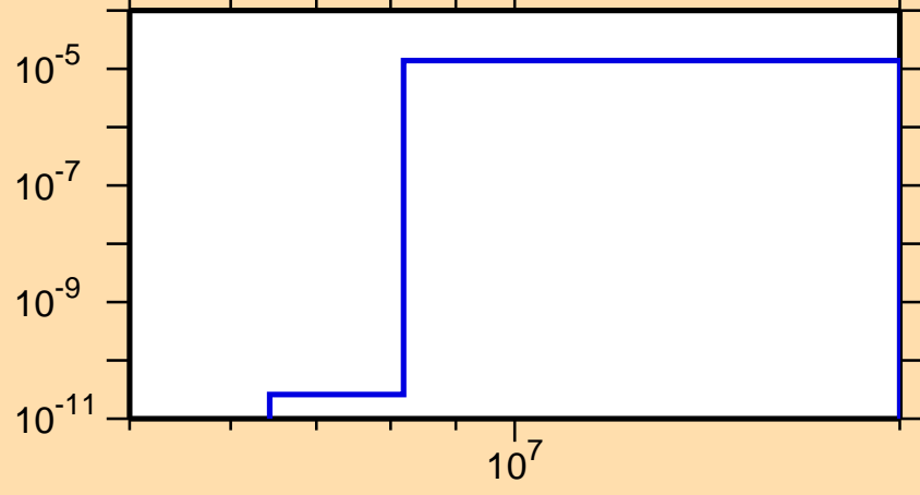
\sigma vs. E for ^{209}\text{Pb}(n,n\alpha)
