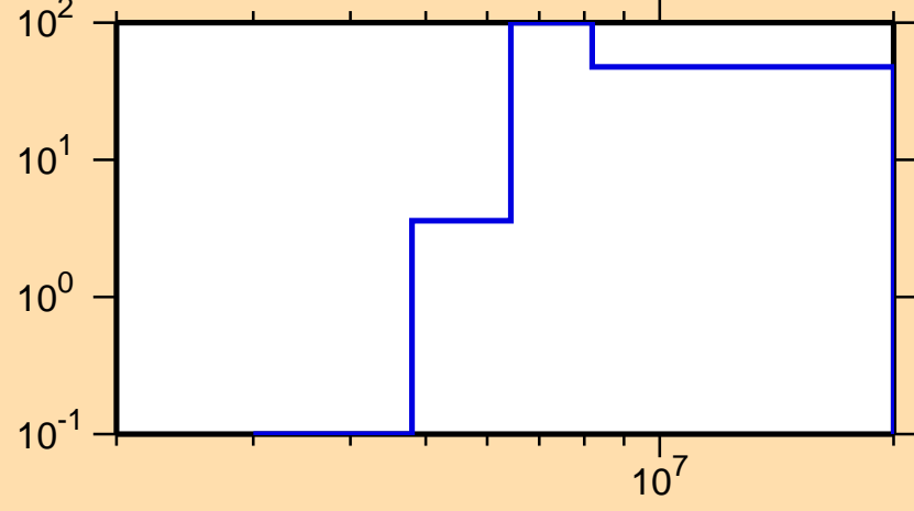
\Delta\sigma/\sigma vs. E for ^{209}\text{Pb}(n,p)
