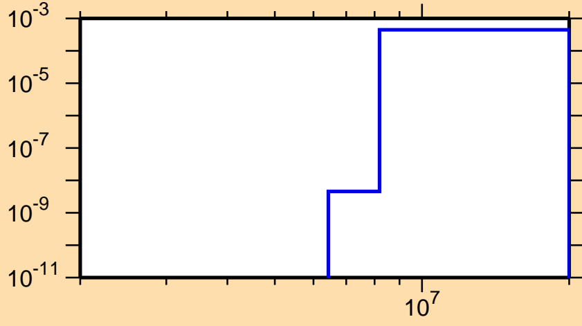
\sigma vs. E for ^{209}\text{Pb}(n,p)
