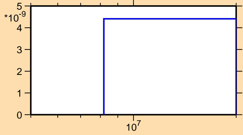
\sigma vs. E for ^{209}\text{Pb}(n,\text{nt})
