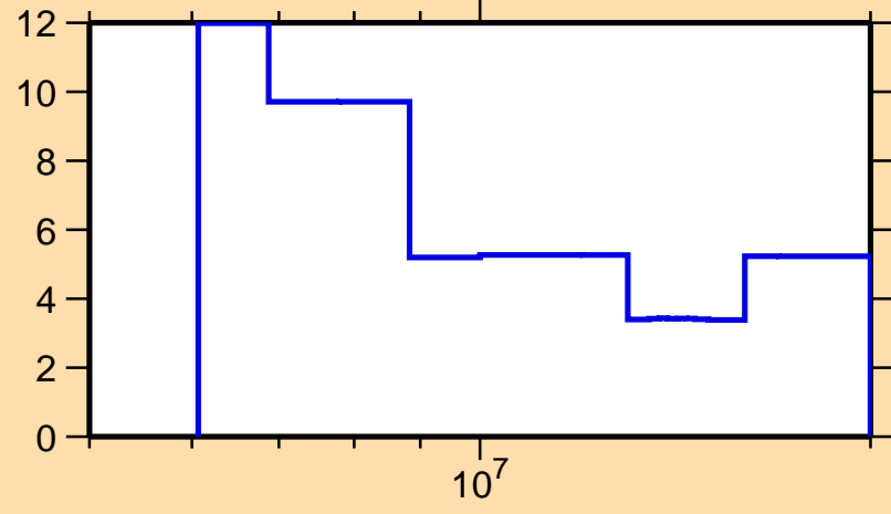
\Delta\sigma/\sigma vs. E for ^{210}\text{Pb}(n,\text{tot.})
