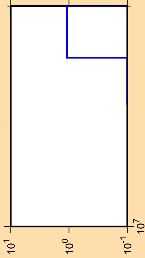
\Delta\sigma/\sigma vs. E for ^{210}\text{Pb} (mt 11)
