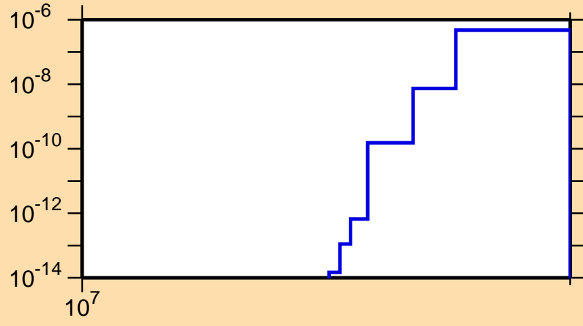
\sigma vs. E for ^{210}\text{Pb}(n,\text{nd})
