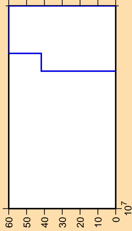
\Delta\sigma/\sigma vs. E for ^{210}\text{Pb}(n,2np)
