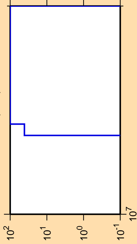
\Delta\sigma/\sigma vs. E for ^{210}\text{Pb}(n,\text{nt})
