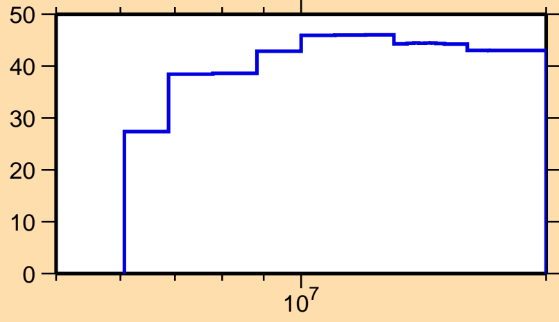
\Delta\sigma/\sigma vs. E for ^{210}\text{Pb}(n,n\text{cont.})
