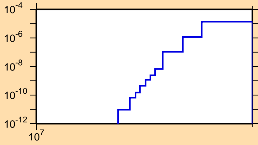
\sigma vs. E for ^{210}\text{Pb}(n,\text{nt})
