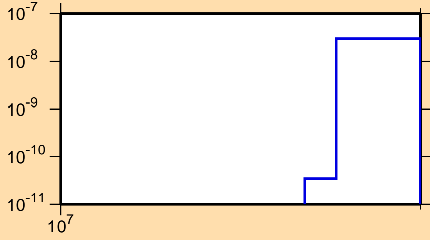
\sigma vs. E for ^{210}\text{Pb}(n,2np)
