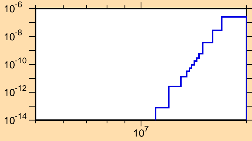
\sigma vs. E for ^{210}\text{Pb}(n,2n\alpha)
