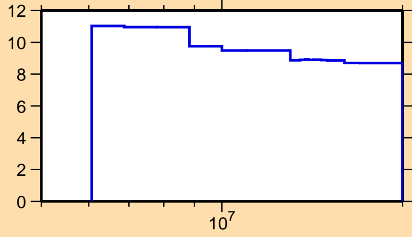
\Delta\sigma/\sigma vs. E for ^{210}\text{Pb}(n,\text{nonel.})
