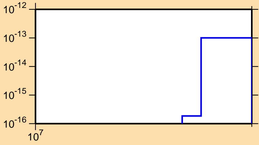
\sigma vs. E for ^{210}\text{Pb}(n,3n\alpha)
