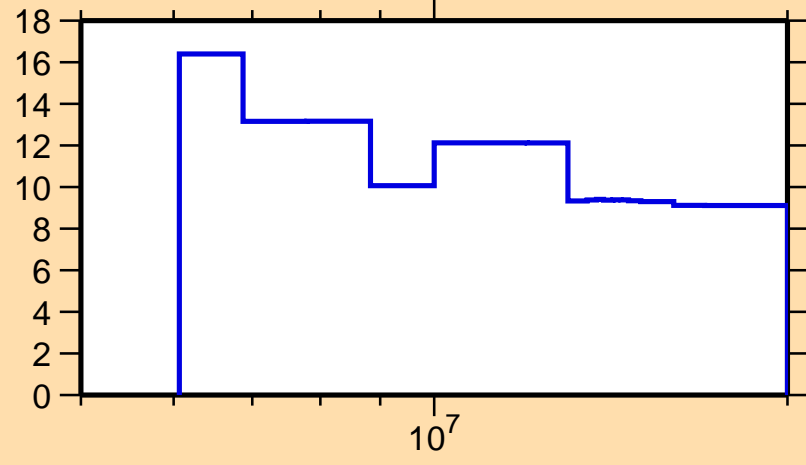
\Delta\sigma/\sigma vs. E for ^{210}\text{Pb}(n,\text{el.})
