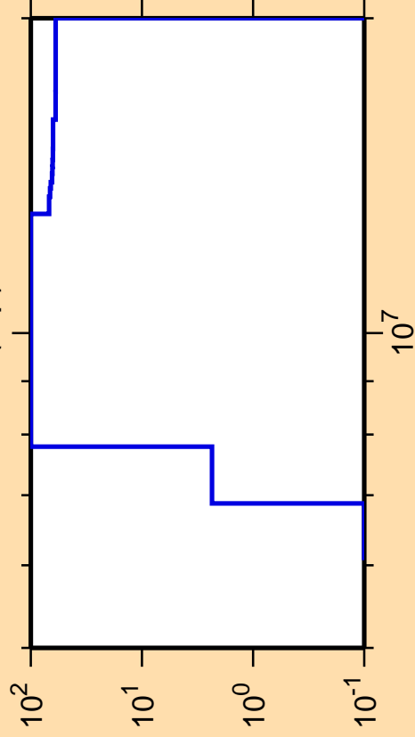
\Delta\sigma/\sigma vs. E for ^{210}\text{Pb}(n,p)
