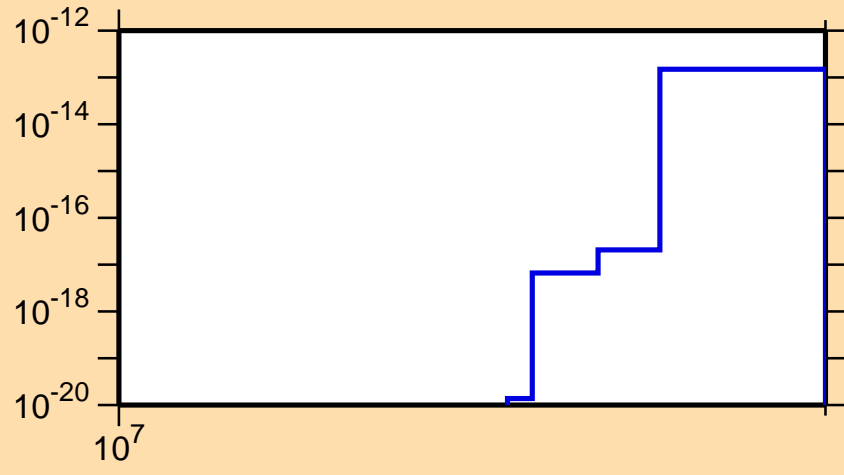
\sigma vs. E for ^{210}\text{Pb} (mt 11)
