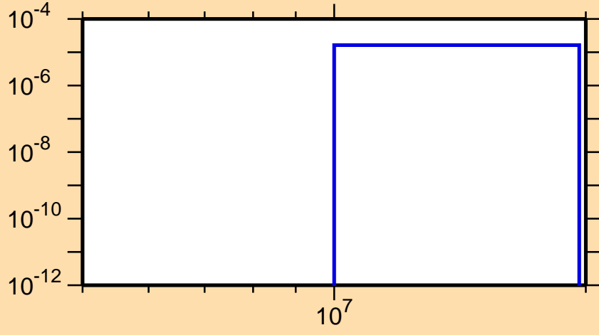
\sigma vs. E for ^{210}\text{Pb}(n,d)
