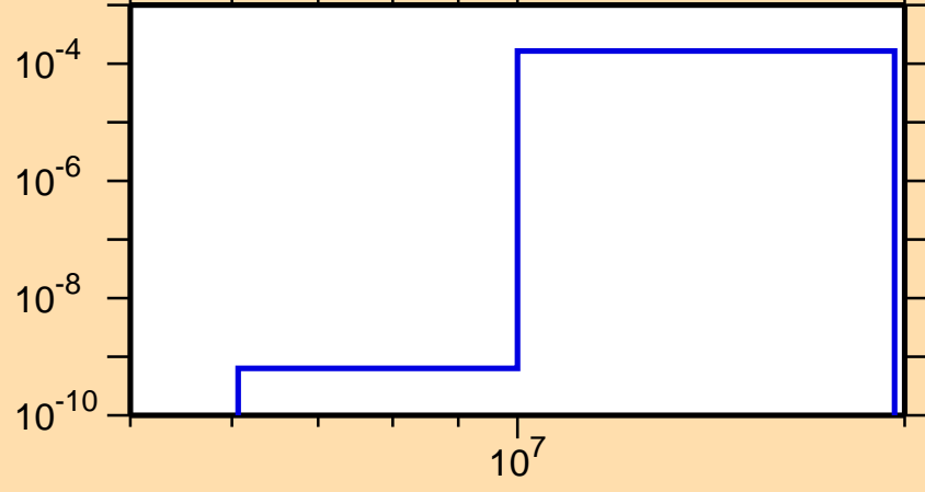
\sigma vs. E for ^{210}\text{Pb}(n,p)
