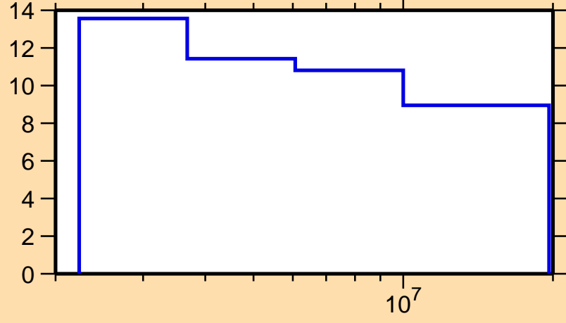
\Delta\sigma/\sigma vs. E for ^{210}\text{Pb}(n,n\text{onel.})
